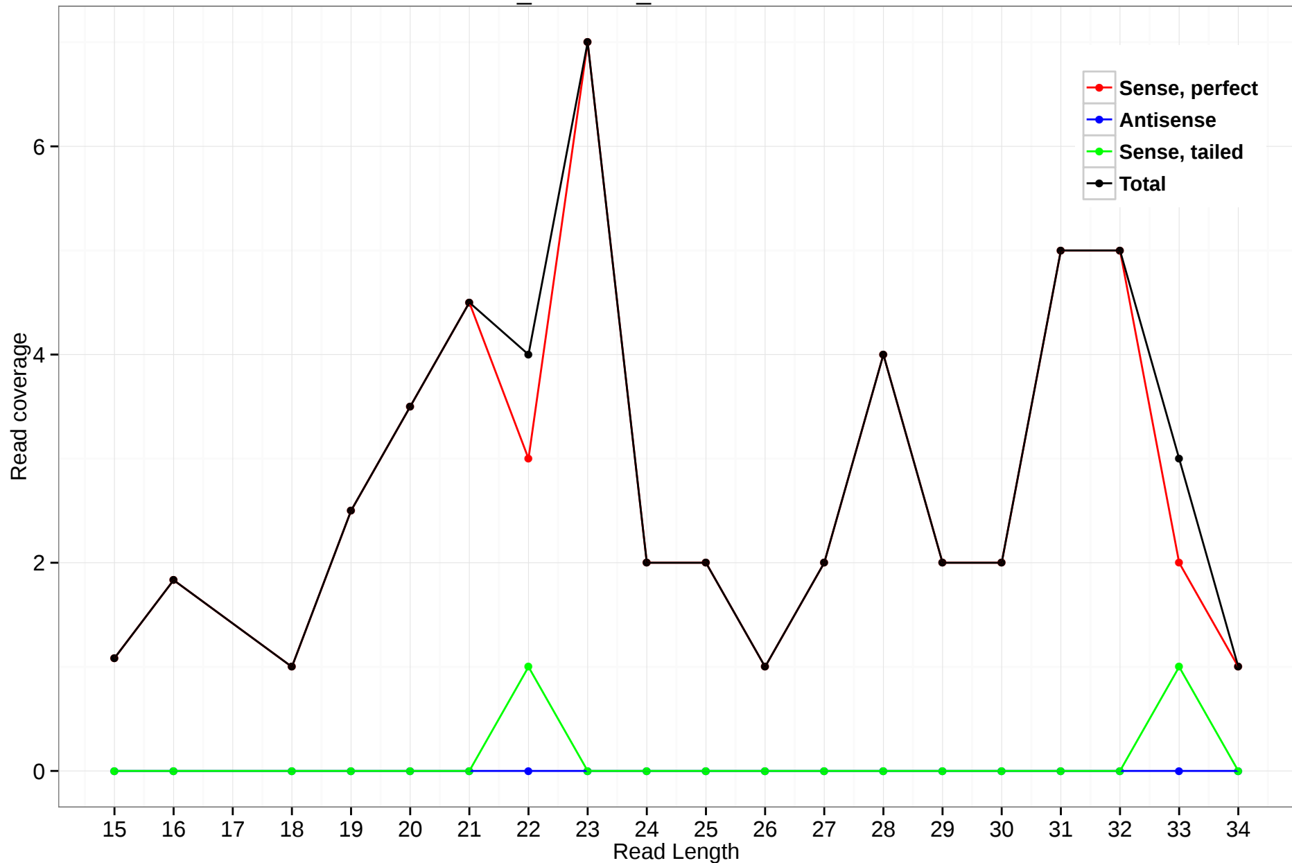
ornAna1_ensGene_ENSOANT00000013780
