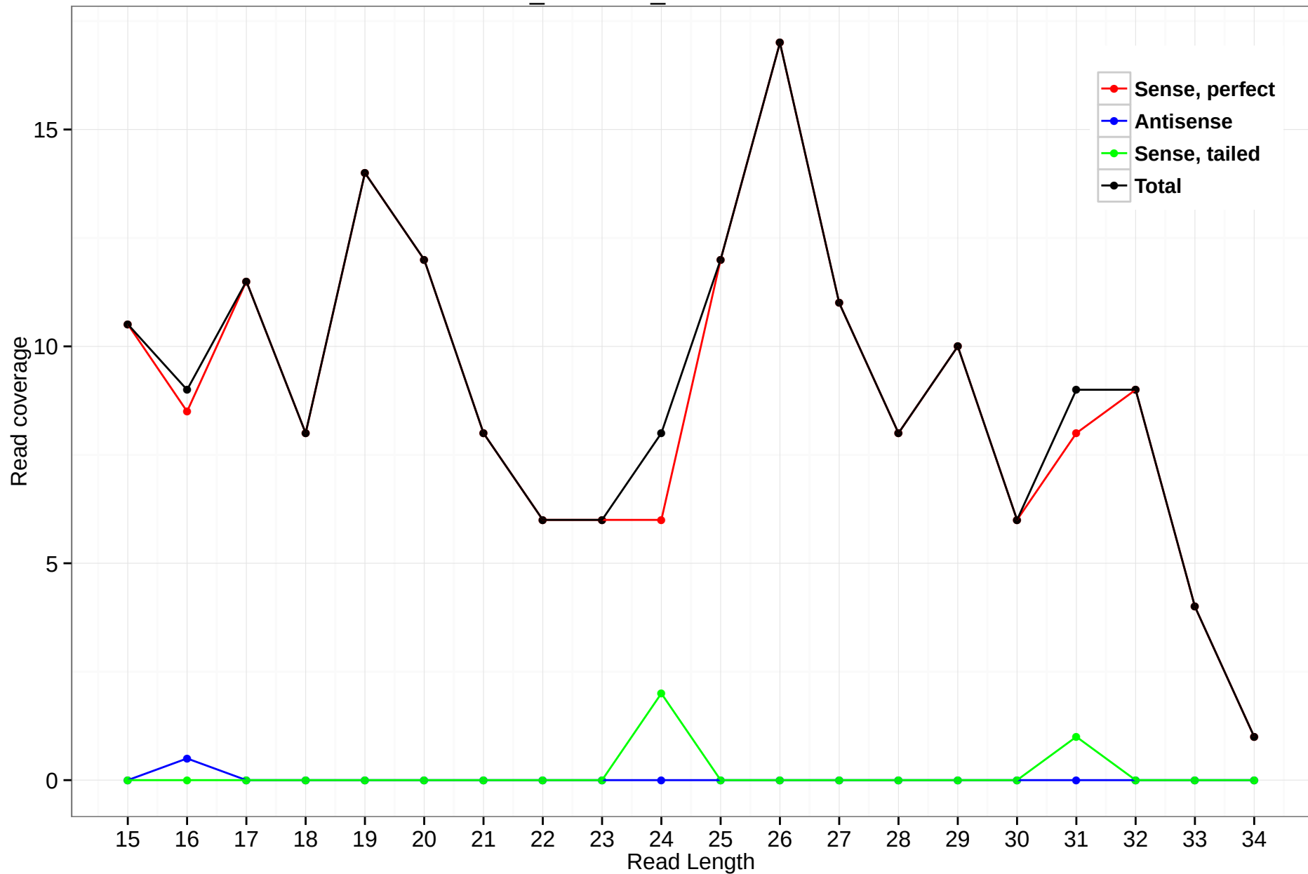
ornAna1_ensGene_ENSOANT00000011421
