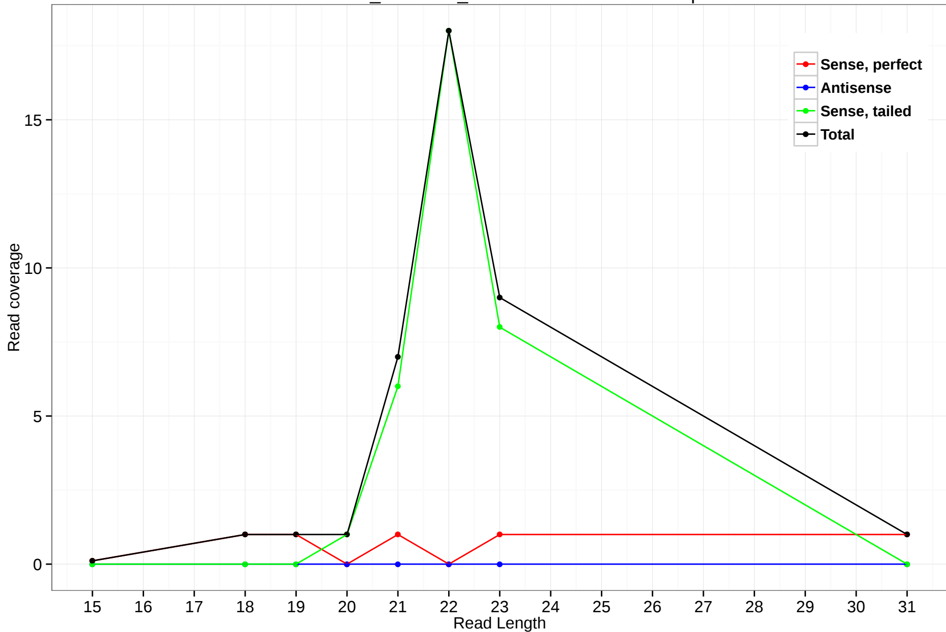
ornAna1_ensGene_ENSOANT00000006087.3p
