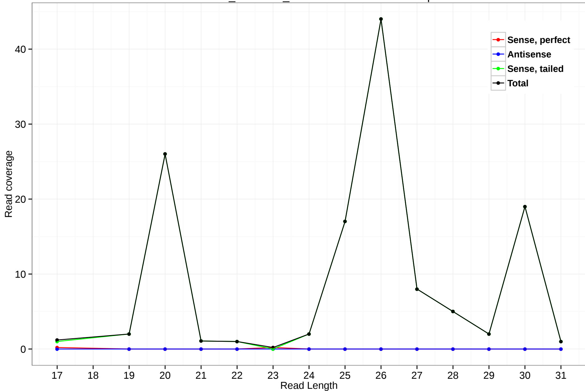
ornAna1_ensGene_ENSOANT00000003751.5p
