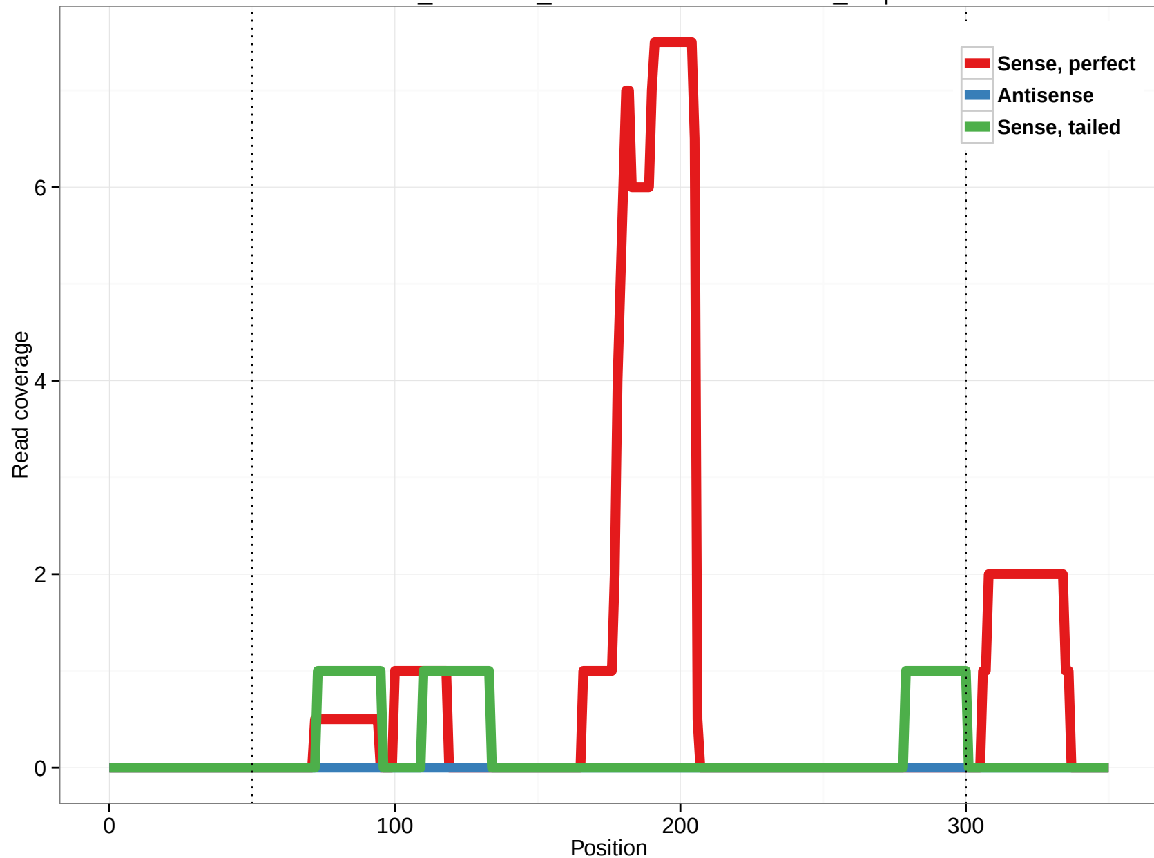
ornAna1_ensGene_ENSOANT00000032806_0.3p
