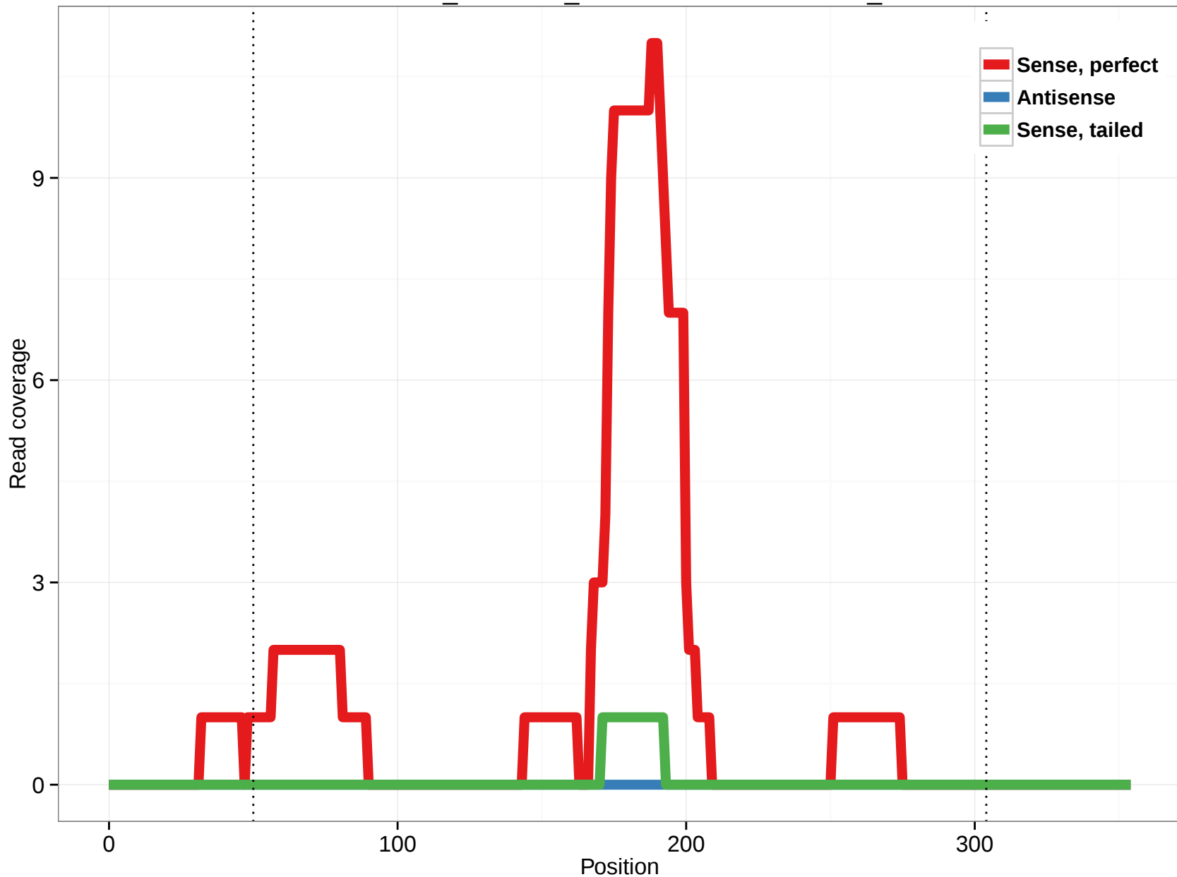
ornAna1_ensGene_ENSOANT00000032748_1
