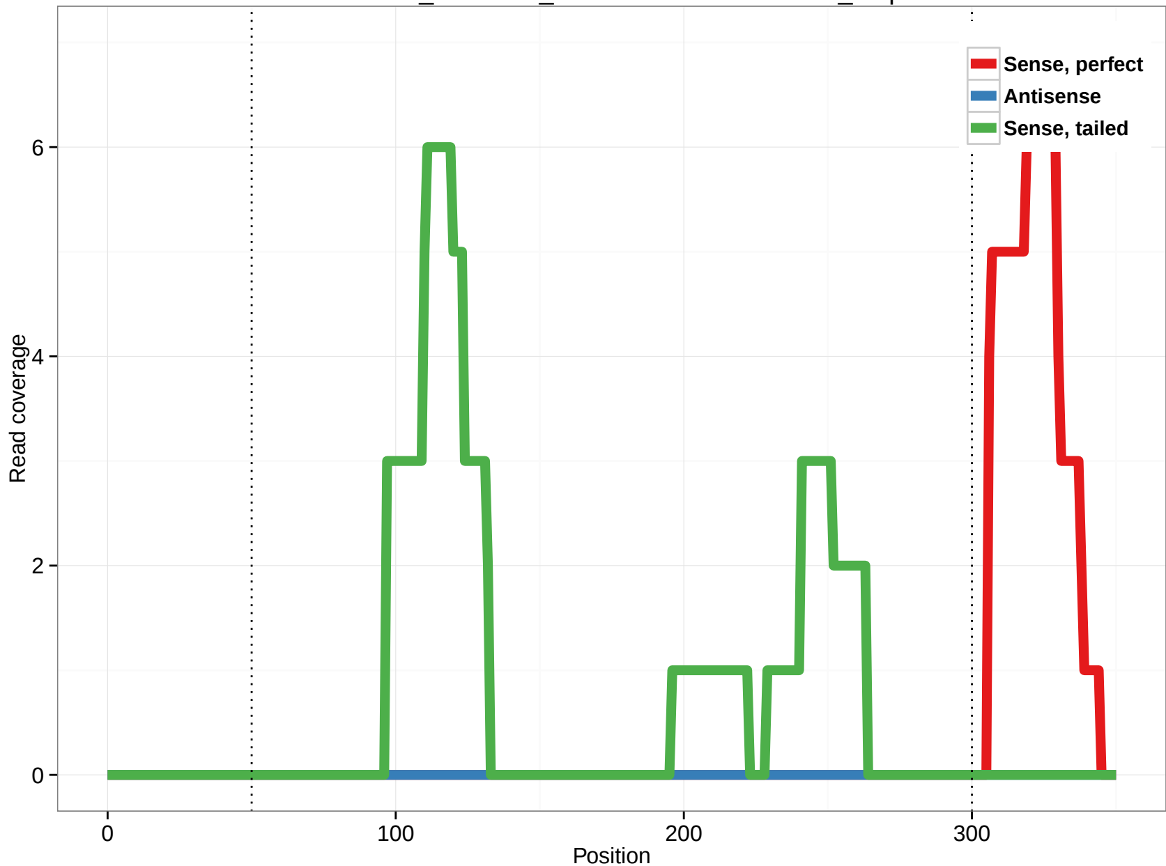
ornAna1_ensGene_ENSOANT00000032743_2.3p
