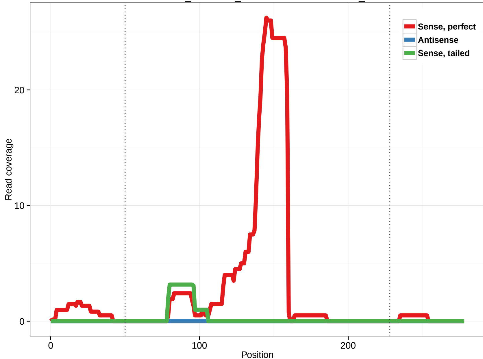
ornAna1_ensGene_ENSOANT00000032730_0
