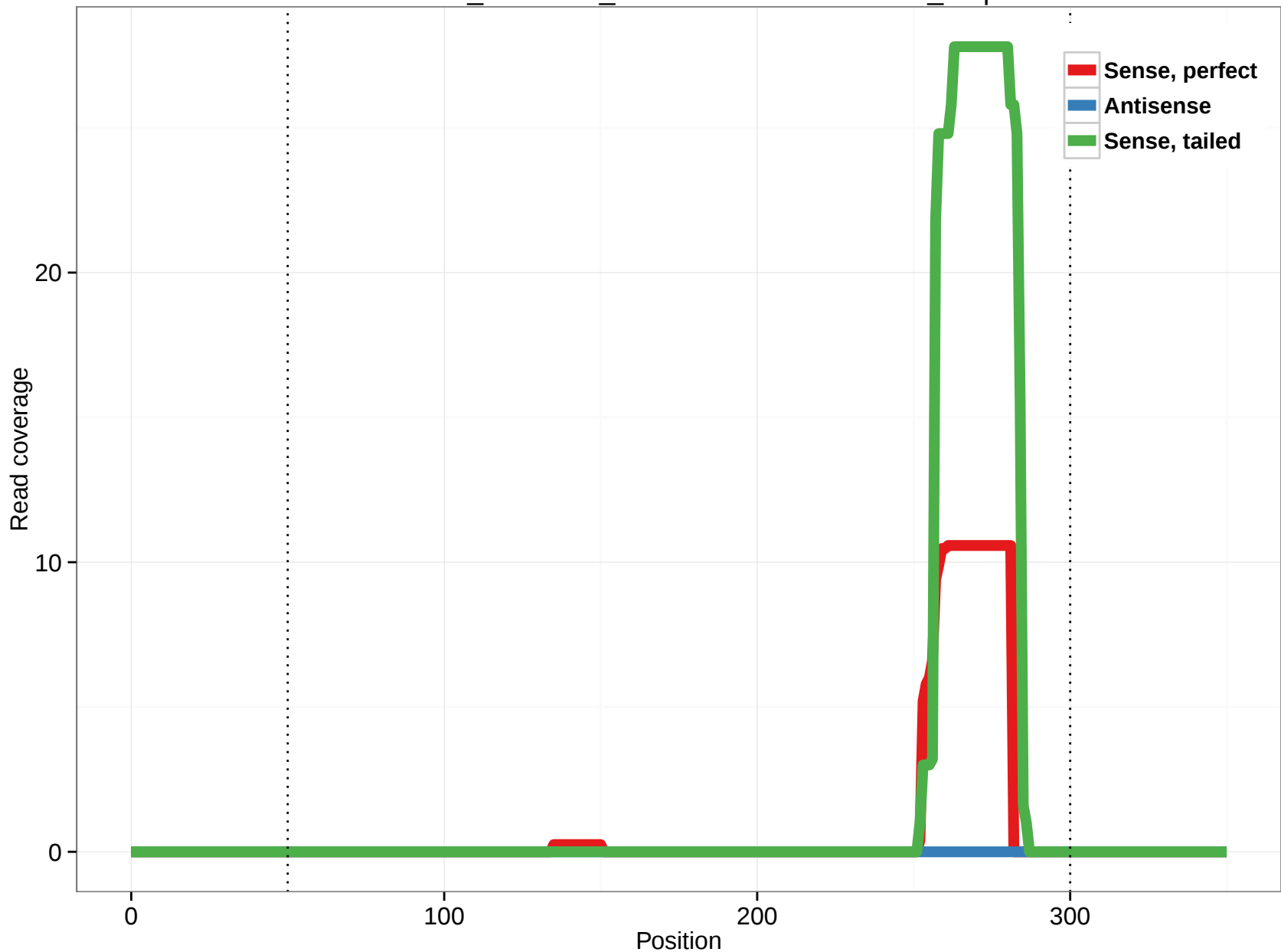
ornAna1_ensGene_ENSOANT00000032659_3.5p
