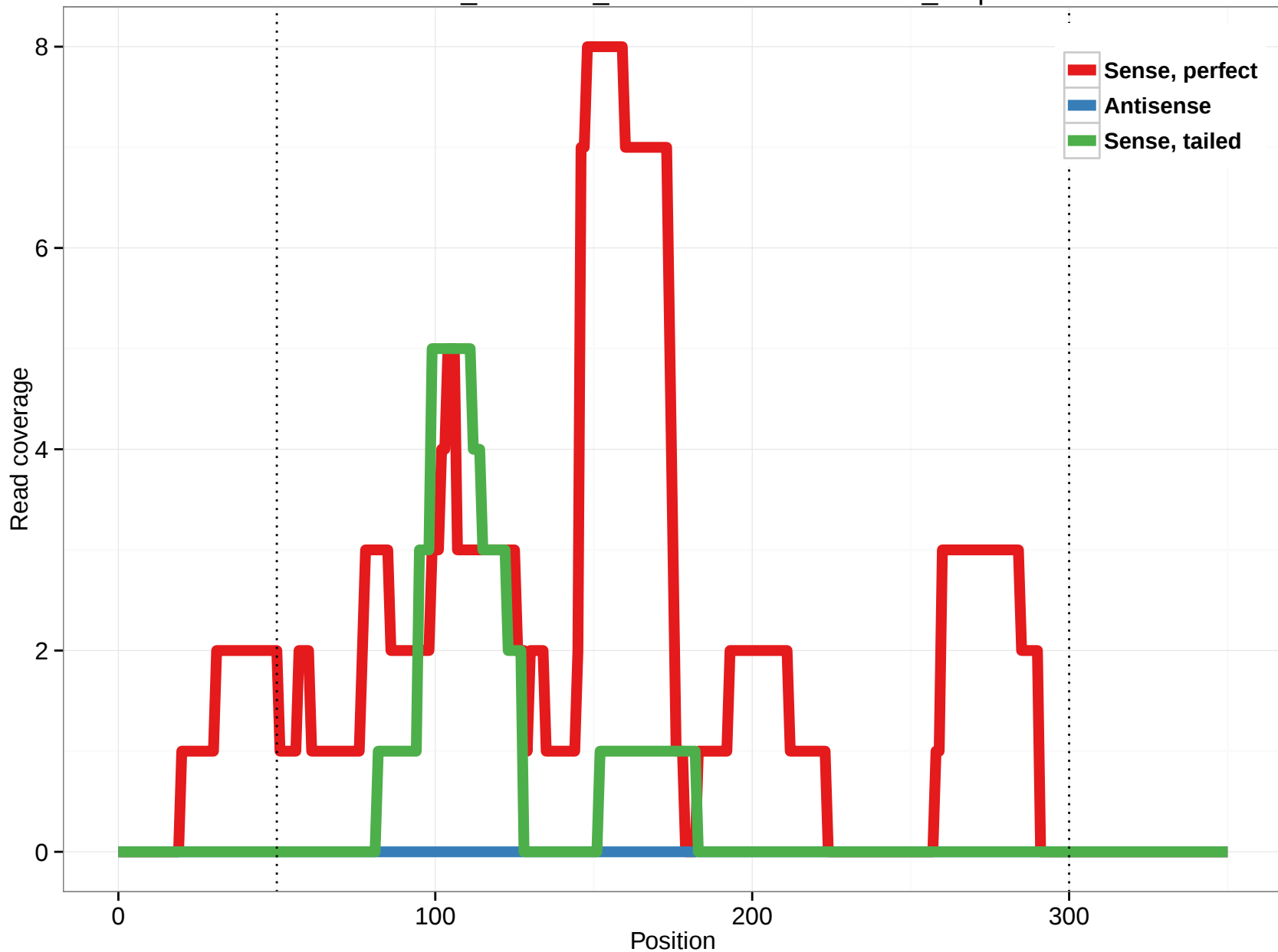
ornAna1_ensGene_ENSOANT00000032556_6.5p
