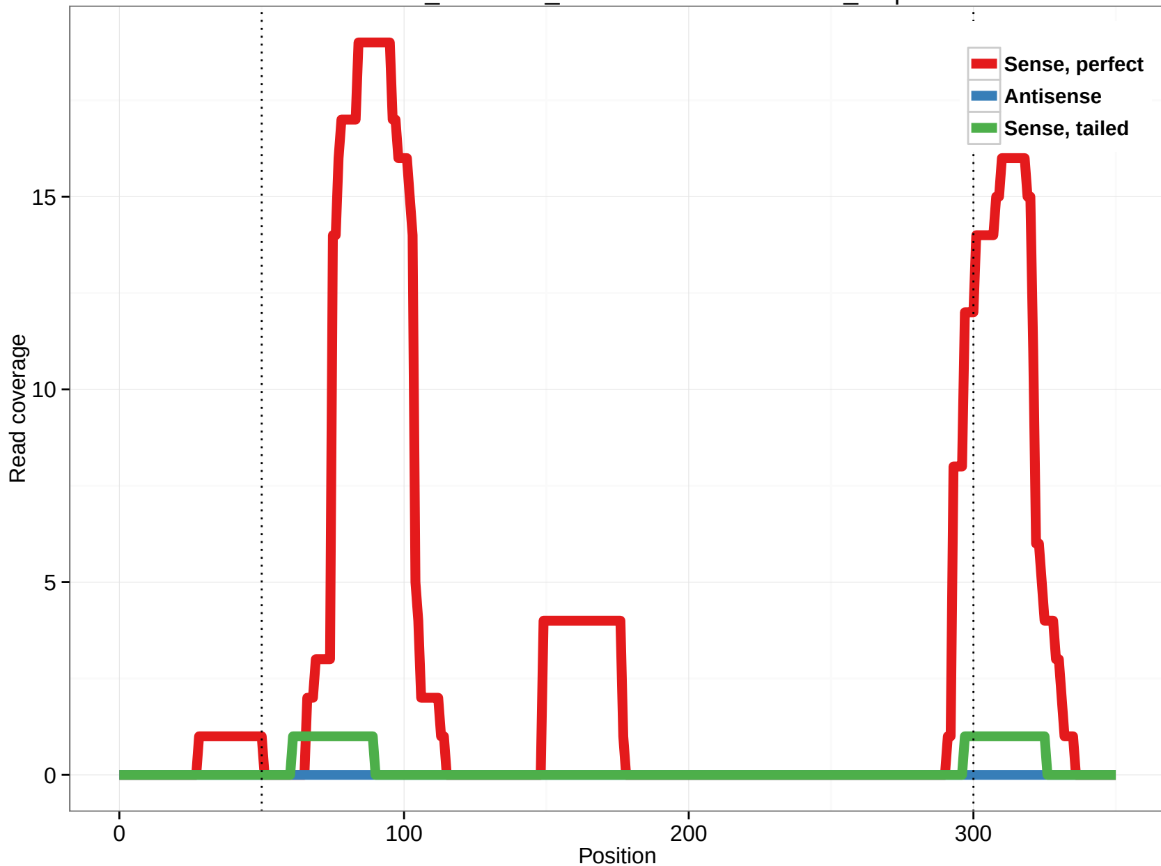
ornAna1_ensGene_ENSOANT00000032556_1.3p
