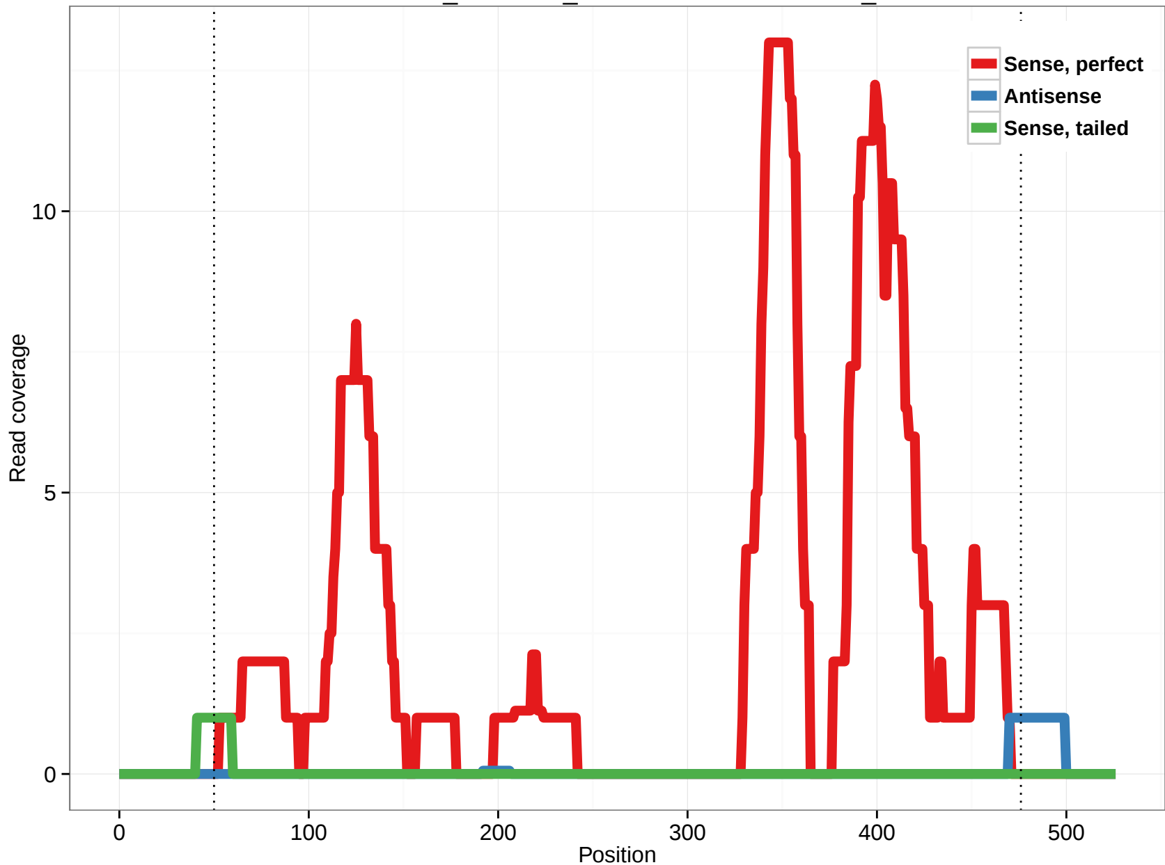
ornAna1_ensGene_ENSOANT00000032517_1
