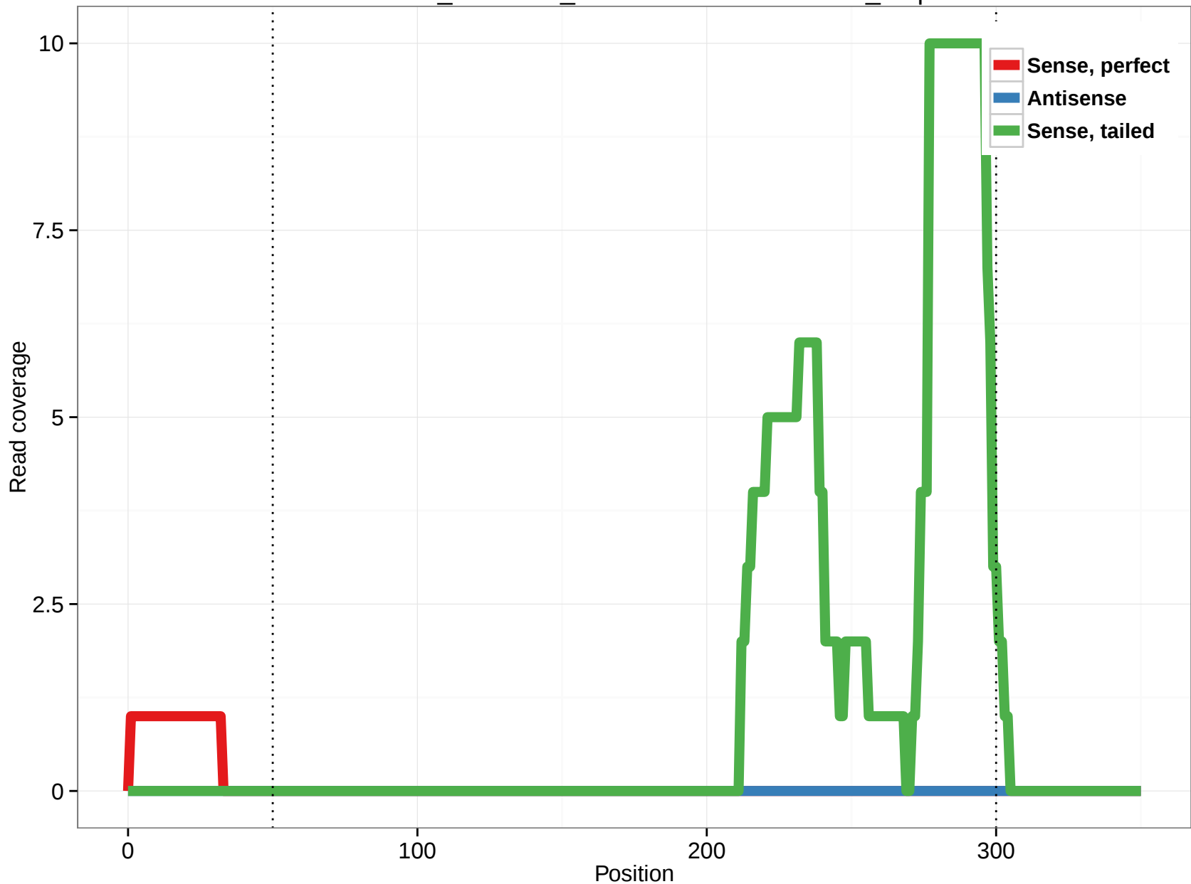
ornAna1_ensGene_ENSOANT00000032506_0.5p
