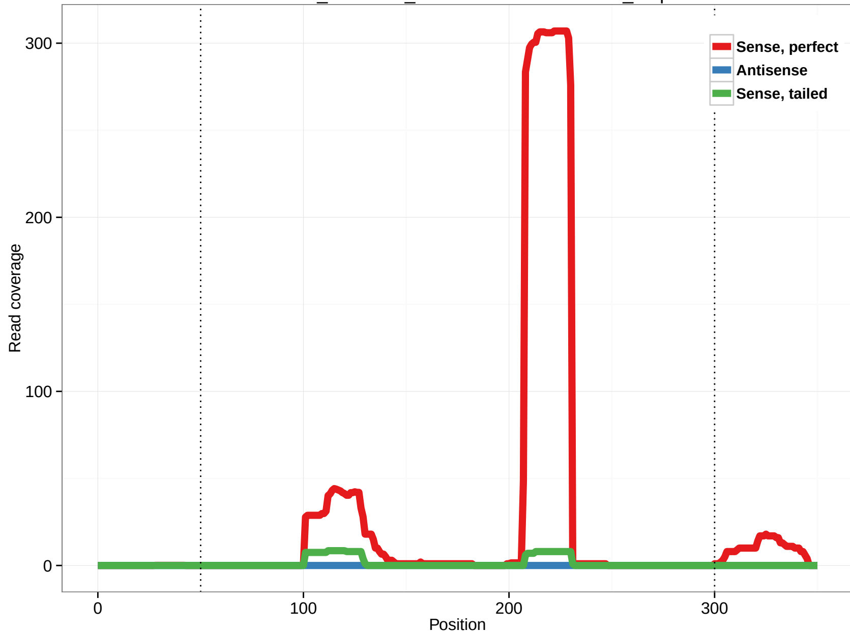
ornAna1_ensGene_ENSOANT00000032470_1.3p
