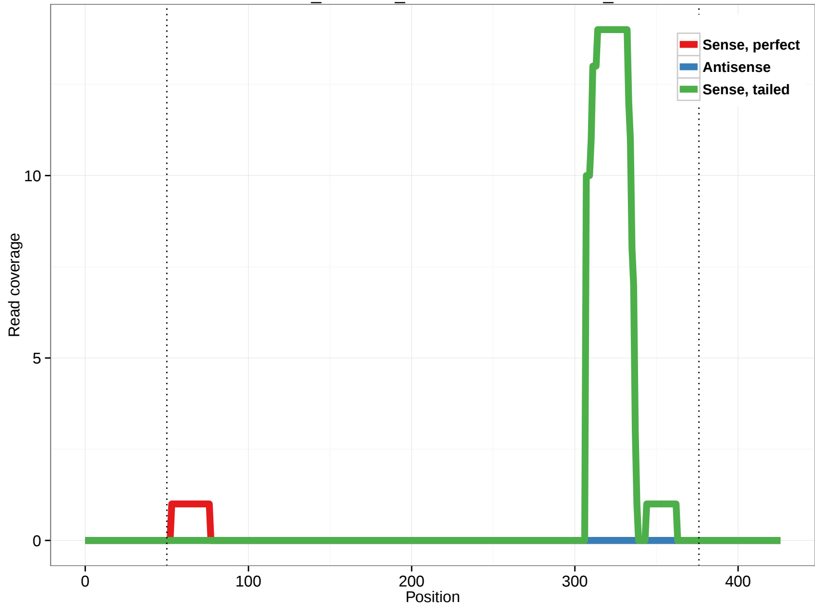
ornAna1_ensGene_ENSOANT00000032306_6
