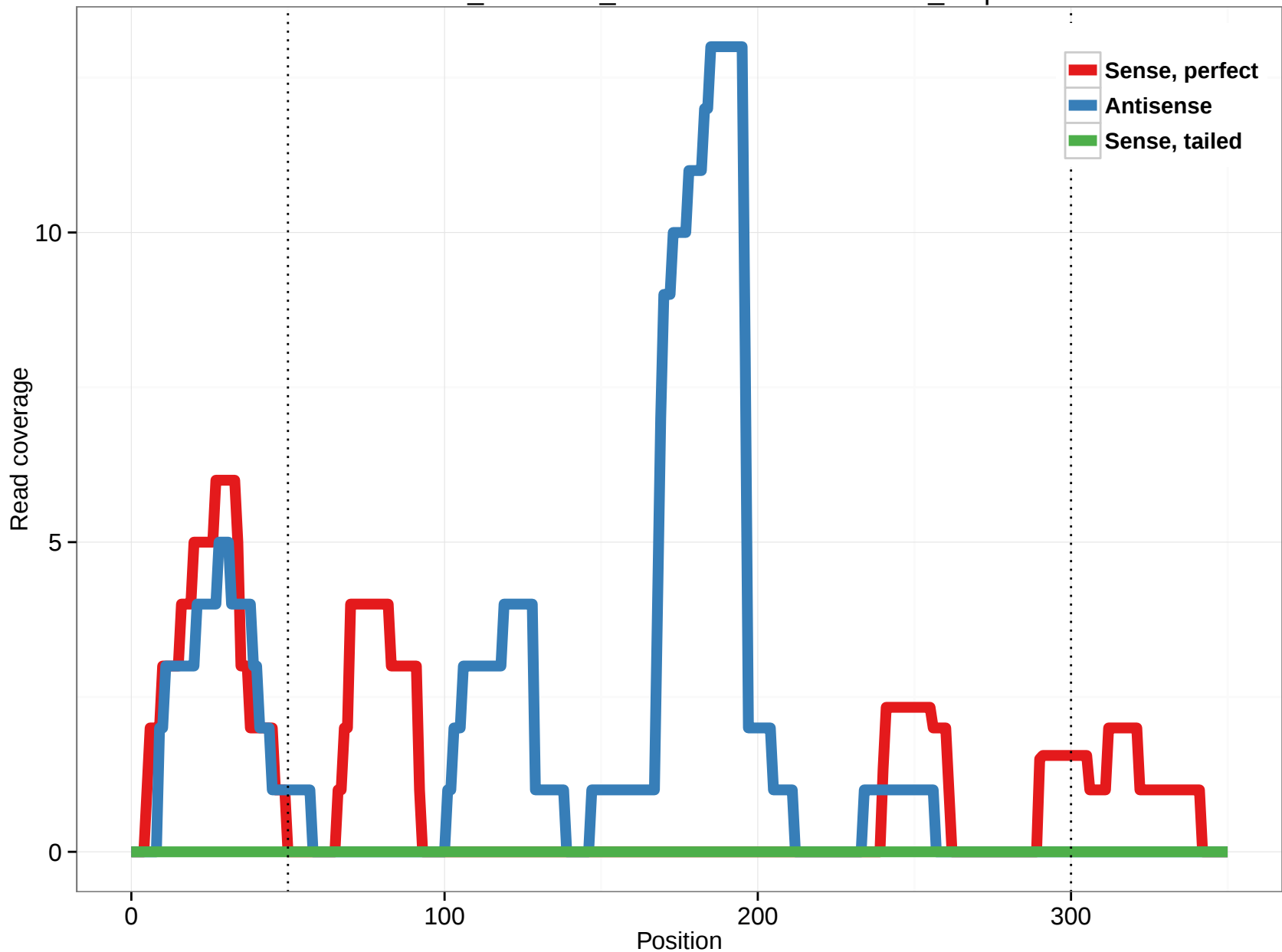
ornAna1_ensGene_ENSOANT00000032268_5.3p
