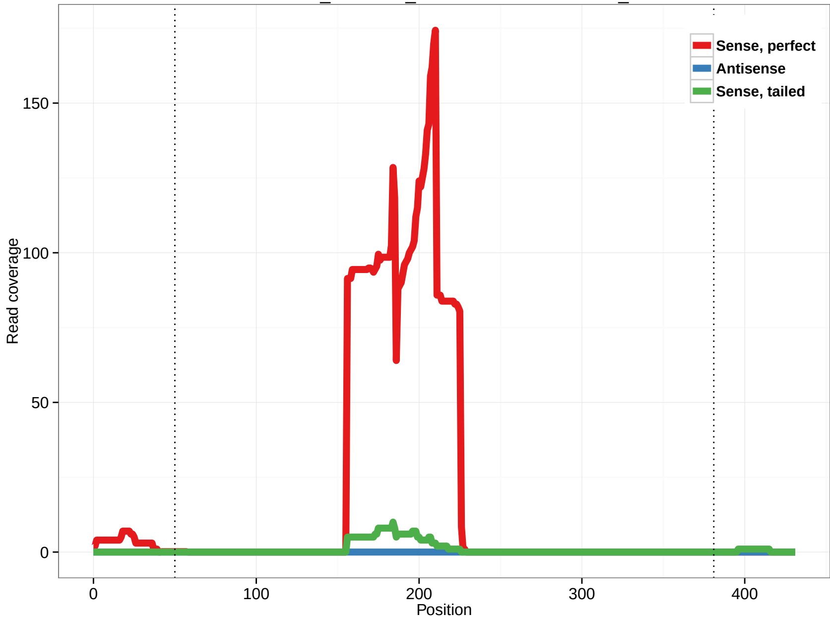
ornAna1_ensGene_ENSOANT00000032227_1
