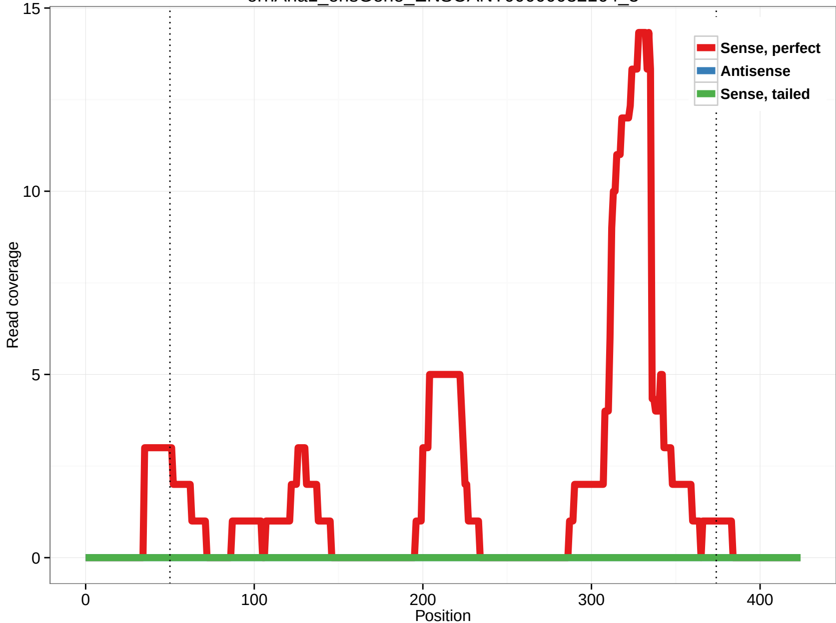
ornAna1_ensGene_ENSOANT00000032164_3
