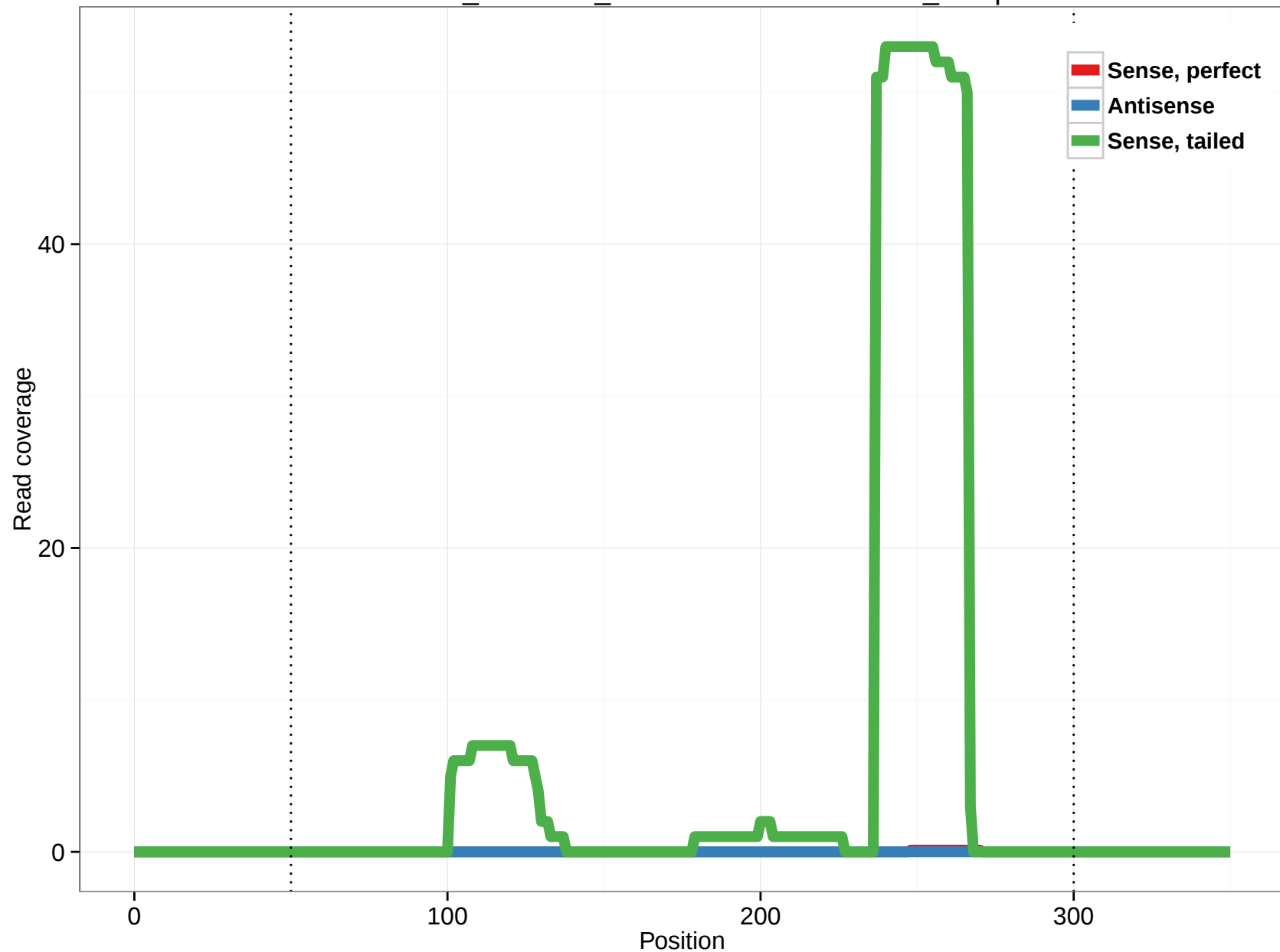
ornAna1_ensGene_ENSOANT00000032078_24.5p
