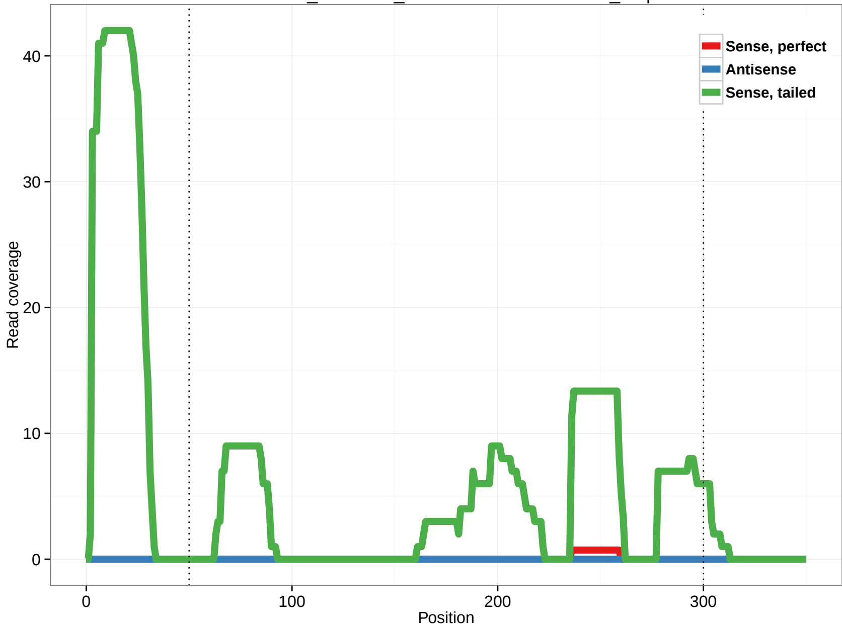
ornAna1_ensGene_ENSOANT00000031761_1.3p
