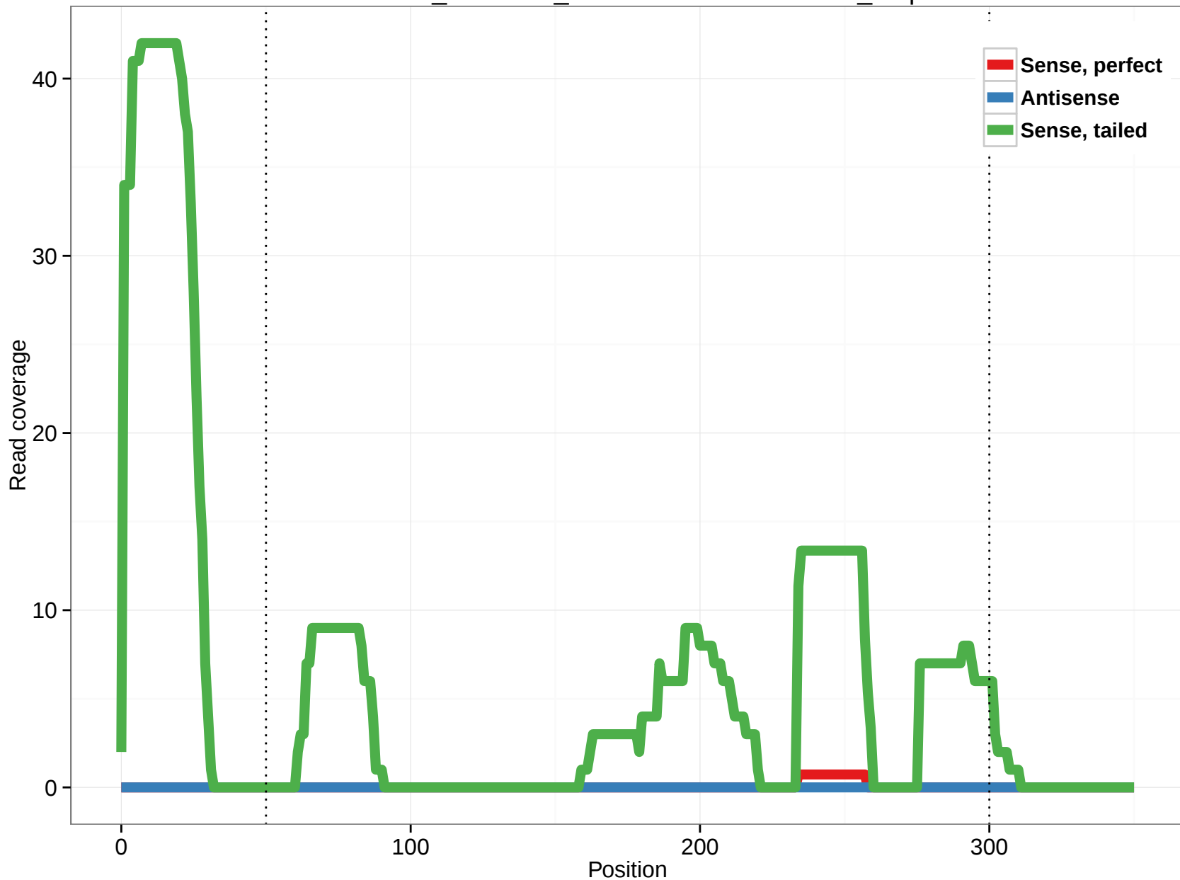
ornAna1_ensGene_ENSOANT00000031760_2.5p
