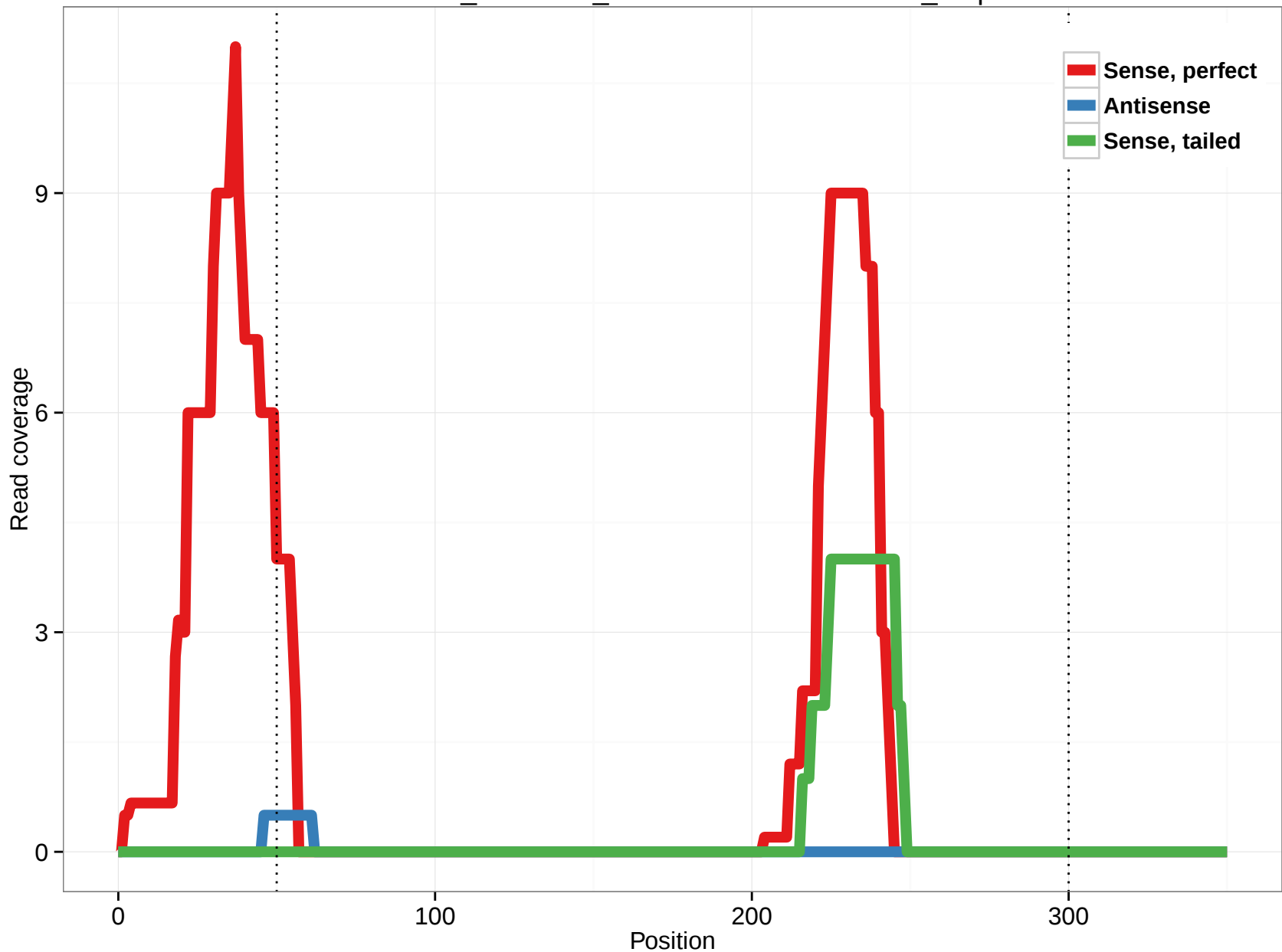
ornAna1_ensGene_ENSOANT00000031743_6.5p
