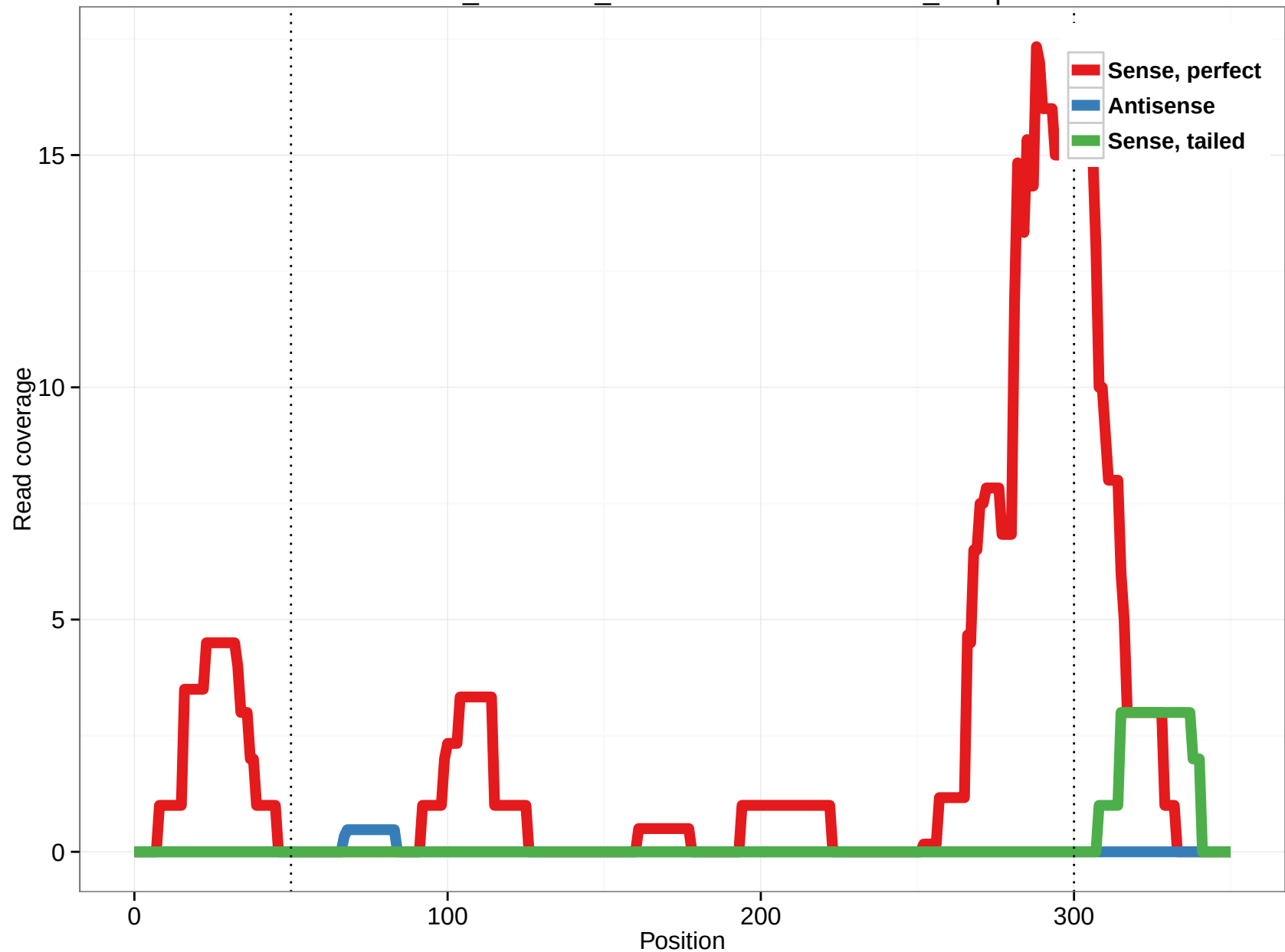
ornAna1_ensGene_ENSOANT00000031738_43.5p
