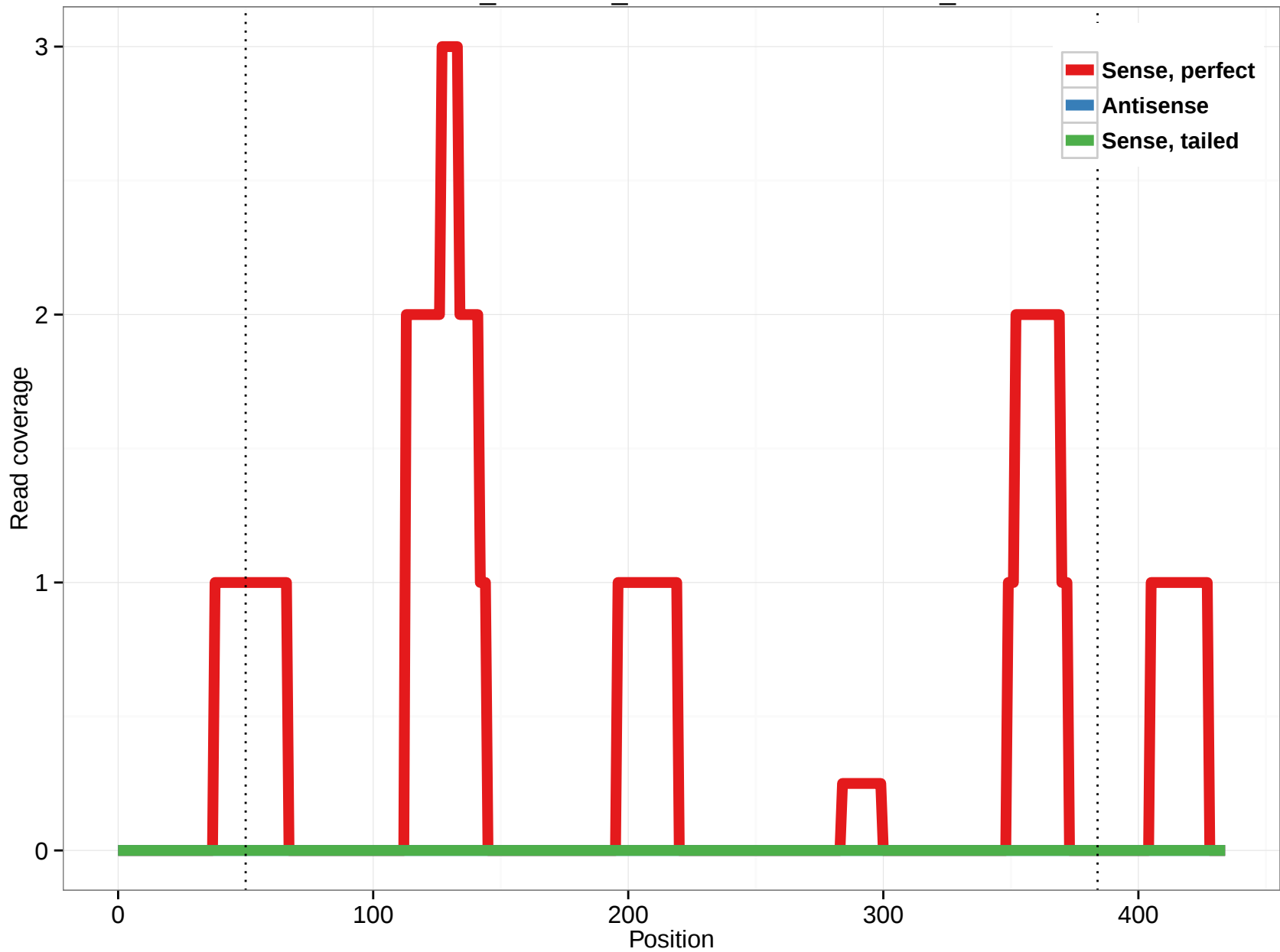
ornAna1_ensGene_ENSOANT00000031478_2
