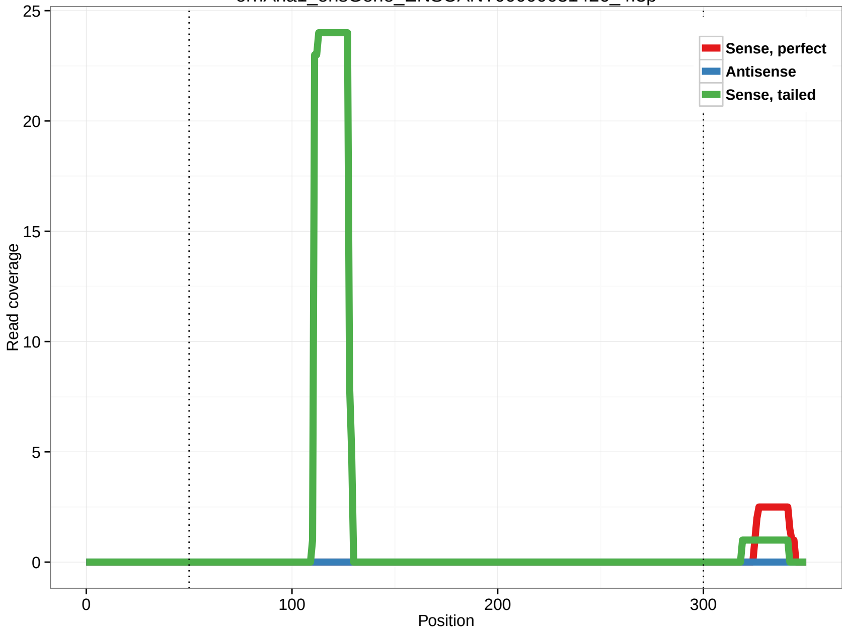
ornAna1_ensGene_ENSOANT00000031426_4.3p
