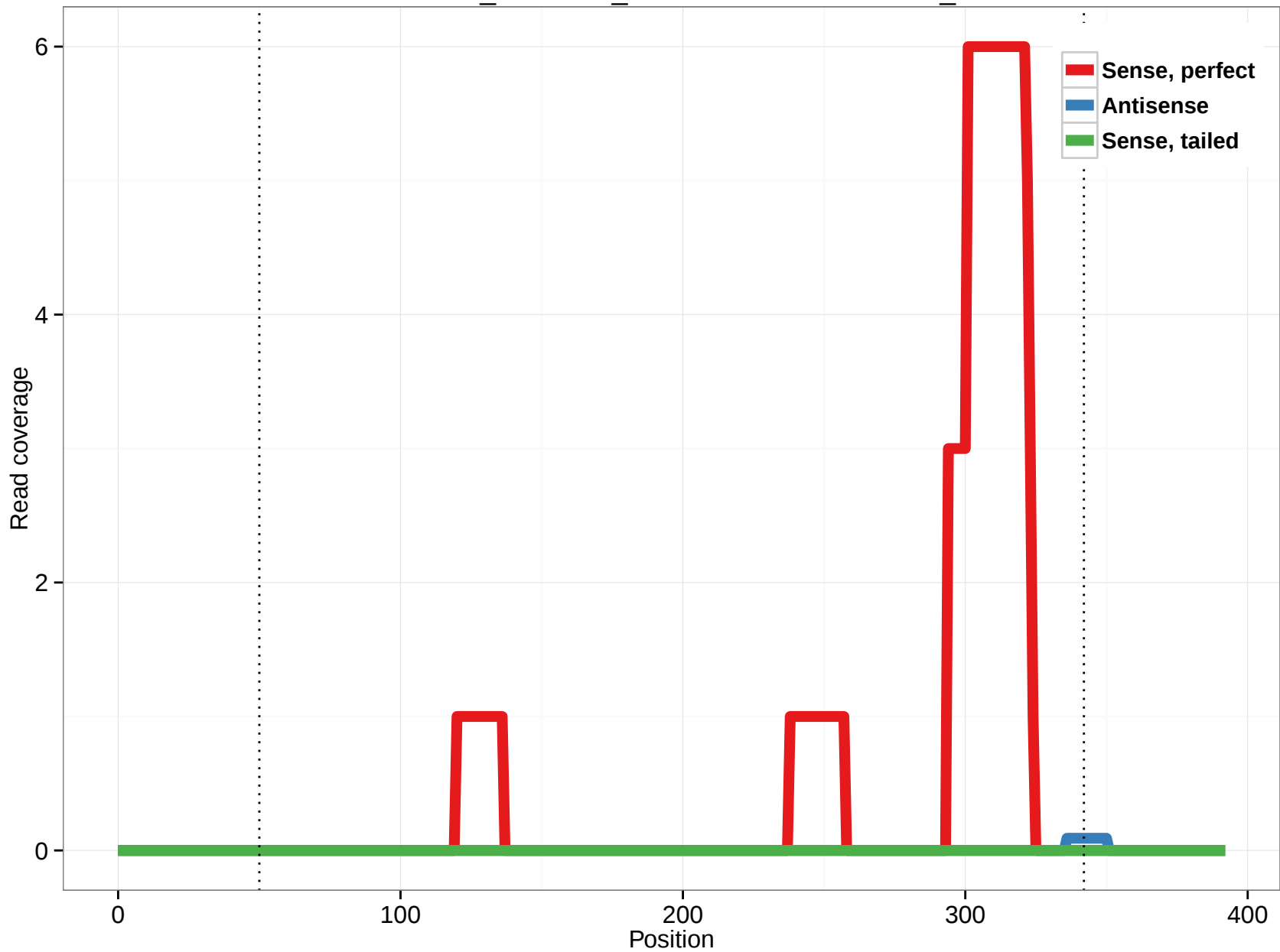
ornAna1_ensGene_ENSOANT00000031178_1
