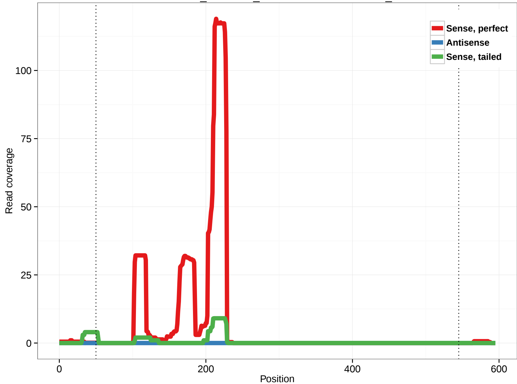
ornAna1_ensGene_ENSOANT00000031081_4
