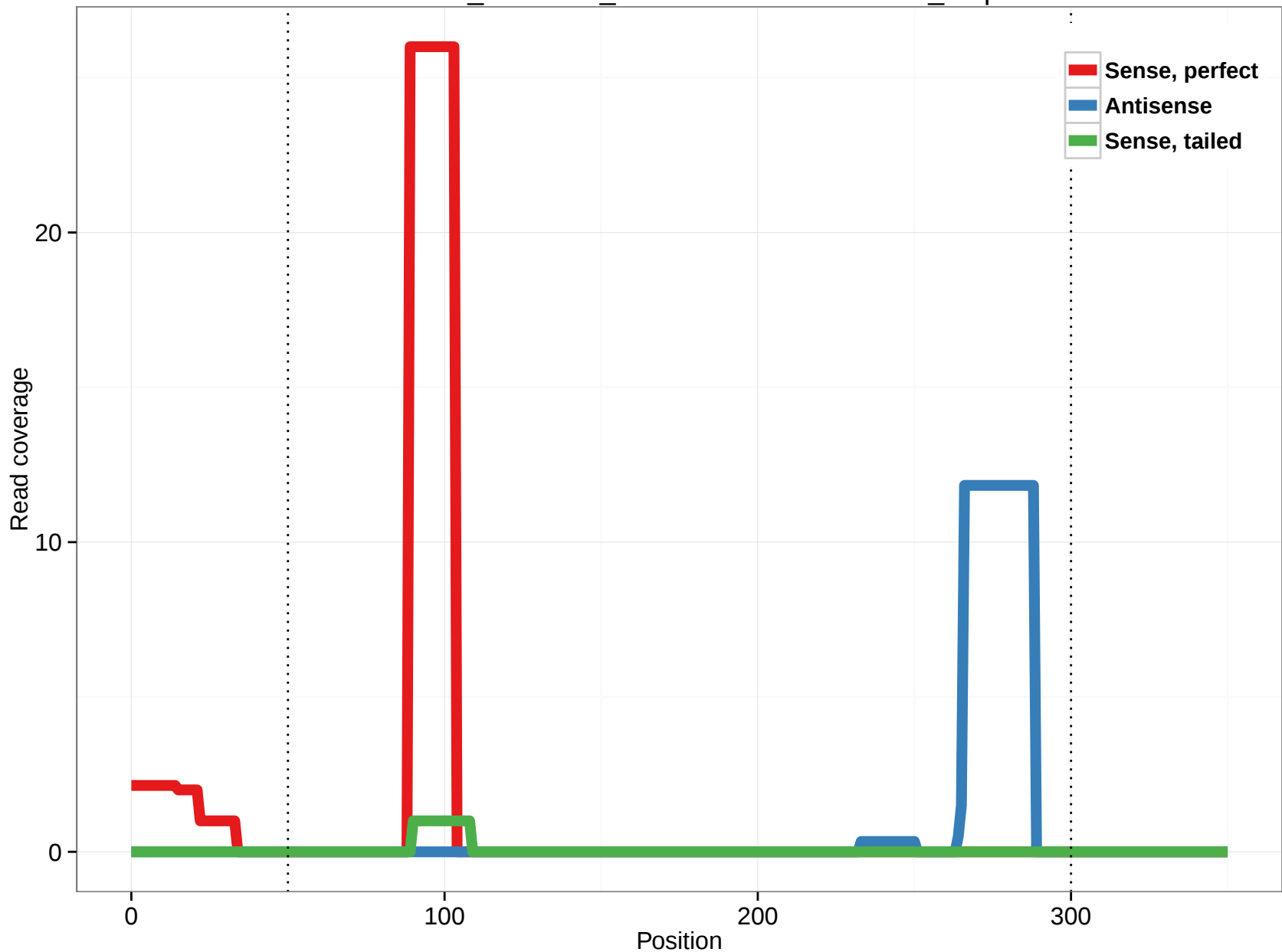
ornAna1_ensGene_ENSOANT00000031034_3.5p
