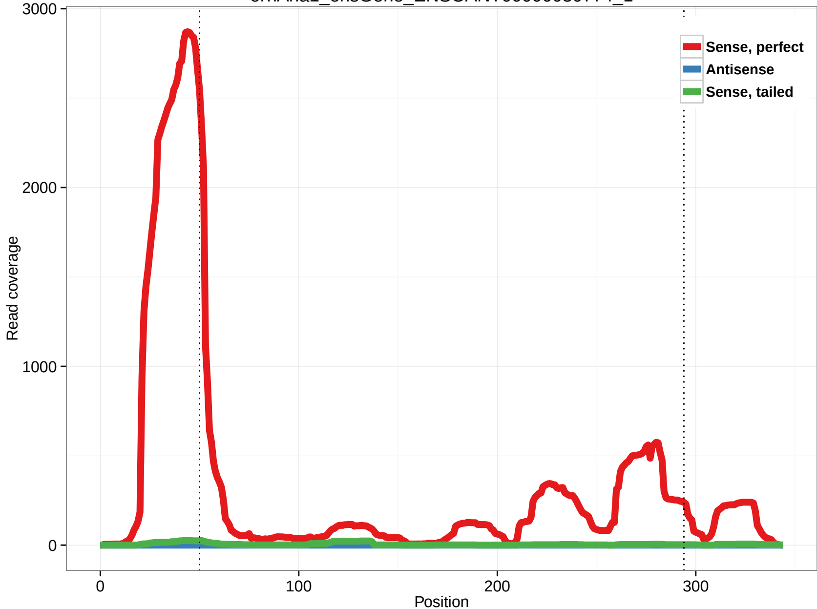
ornAna1_ensGene_ENSOANT00000030774_1
