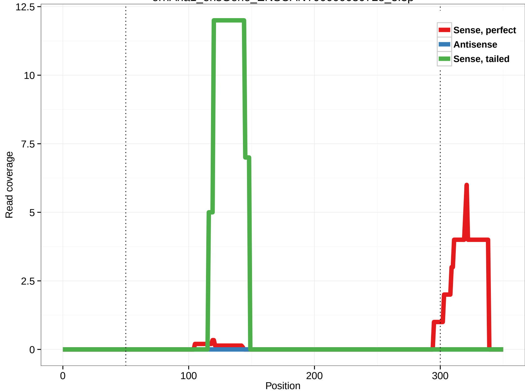
ornAna1_ensGene_ENSOANT00000030728_3.3p
