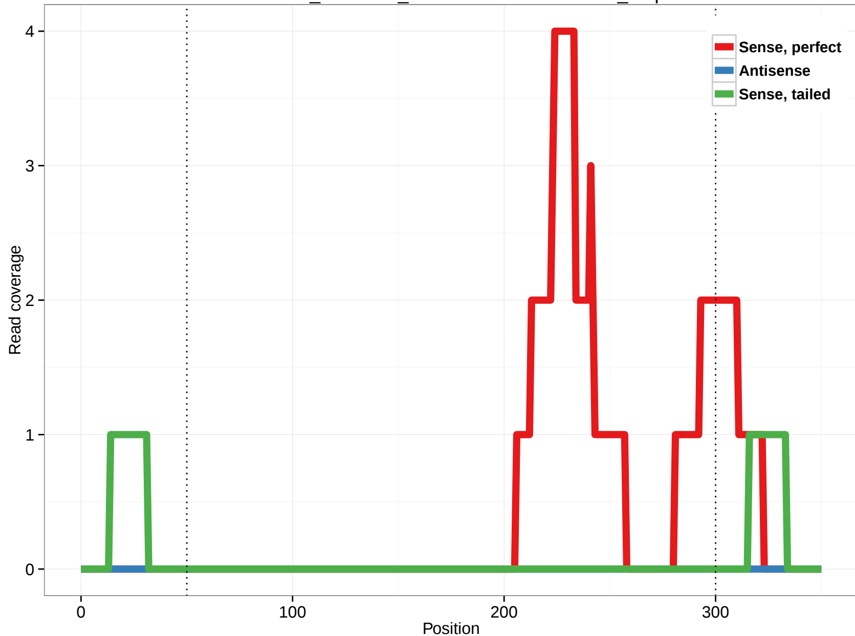
ornAna1_ensGene_ENSOANT00000030650_0.5p
