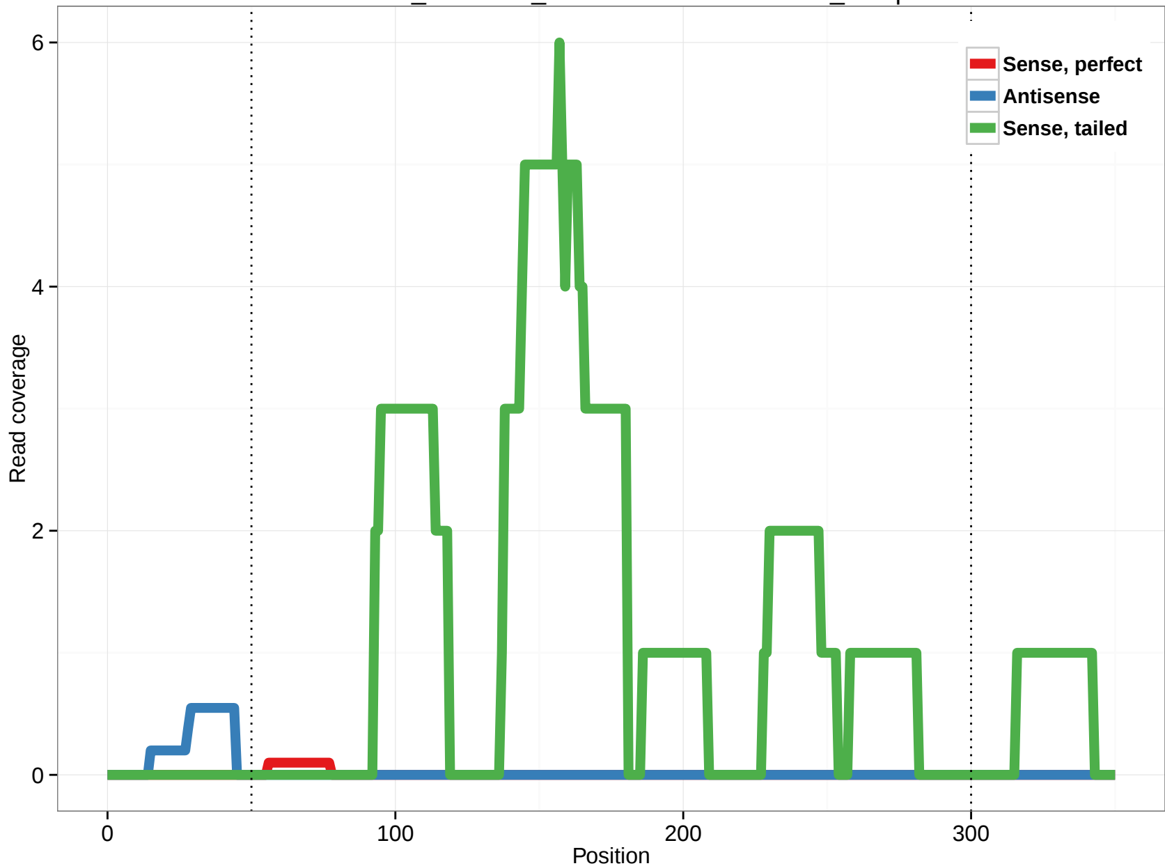
ornAna1_ensGene_ENSOANT00000030609_12.3p
