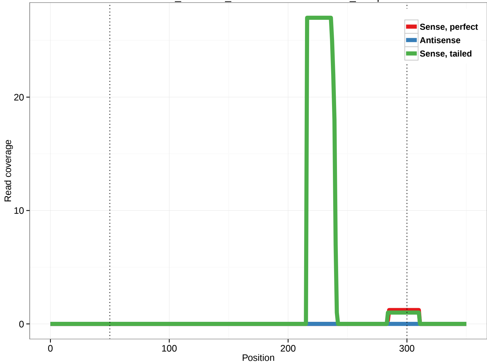
ornAna1_ensGene_ENSOANT00000030575_19.5p
