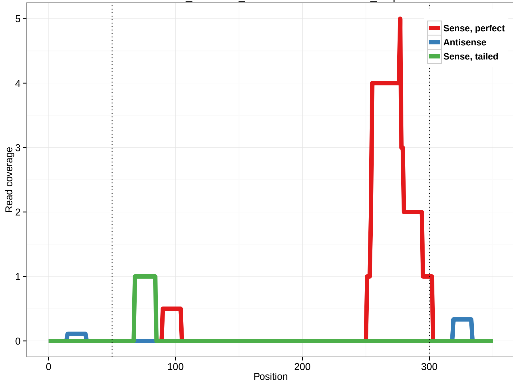
ornAna1_ensGene_ENSOANT00000030566_1.3p
