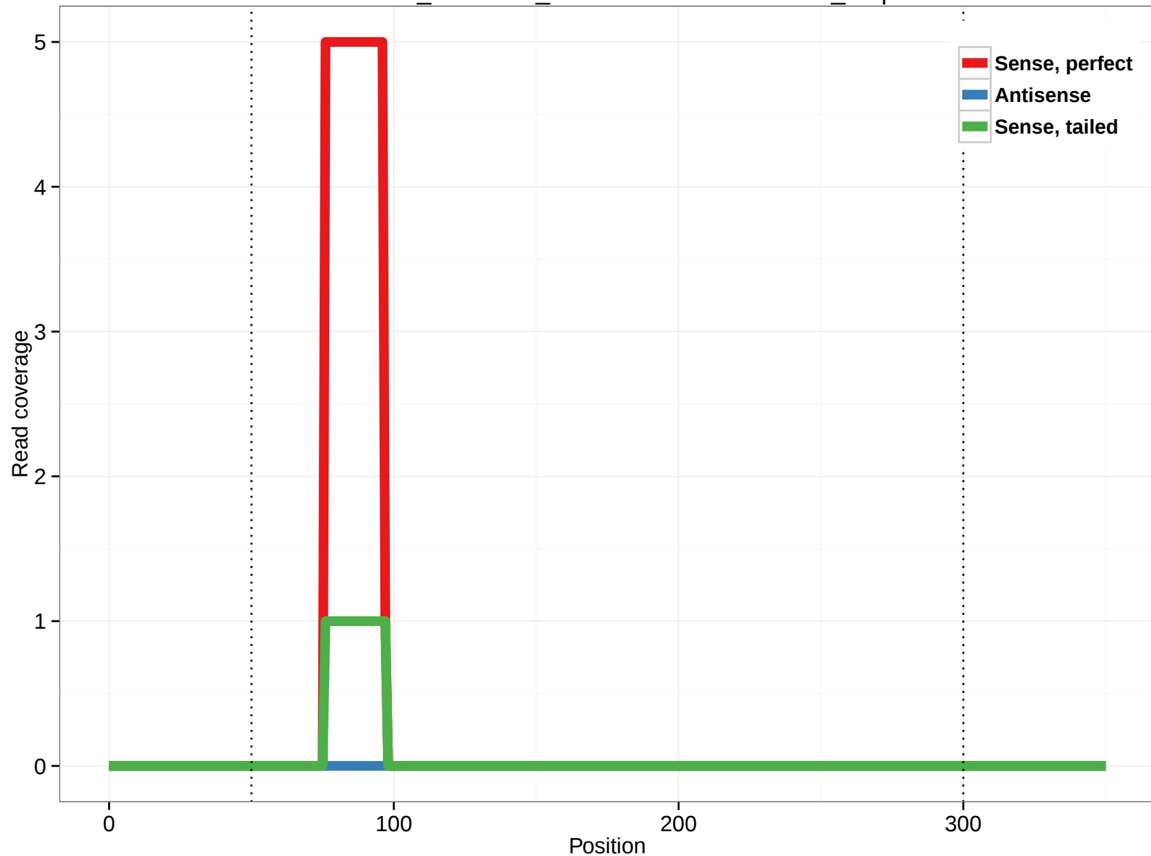
ornAna1_ensGene_ENSOANT00000030383_2.3p
