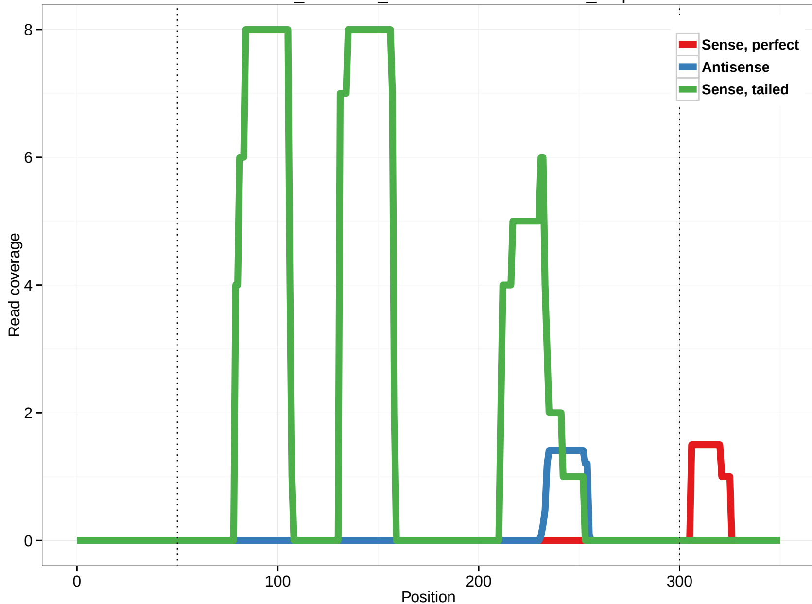
ornAna1_ensGene_ENSOANT00000030298_0.3p
