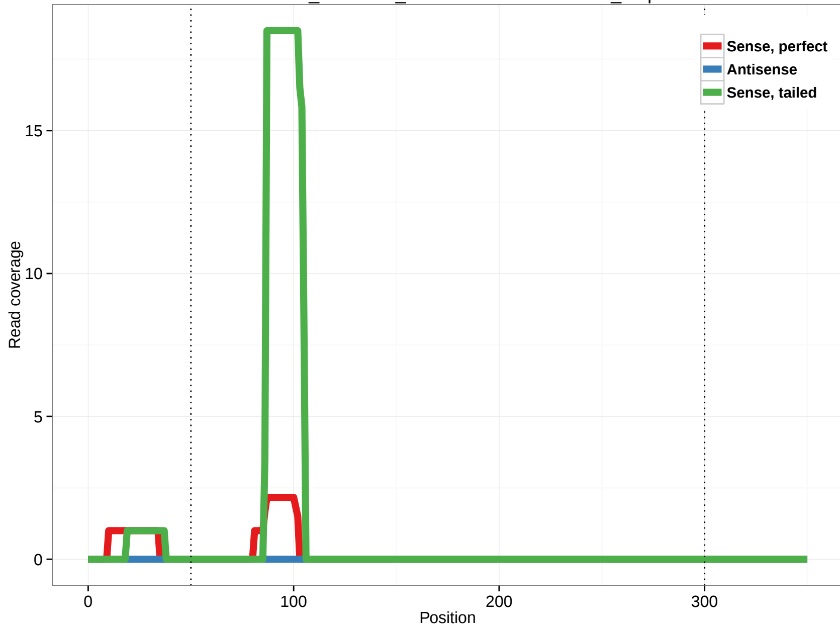
ornAna1_ensGene_ENSOANT00000030223_1.5p
