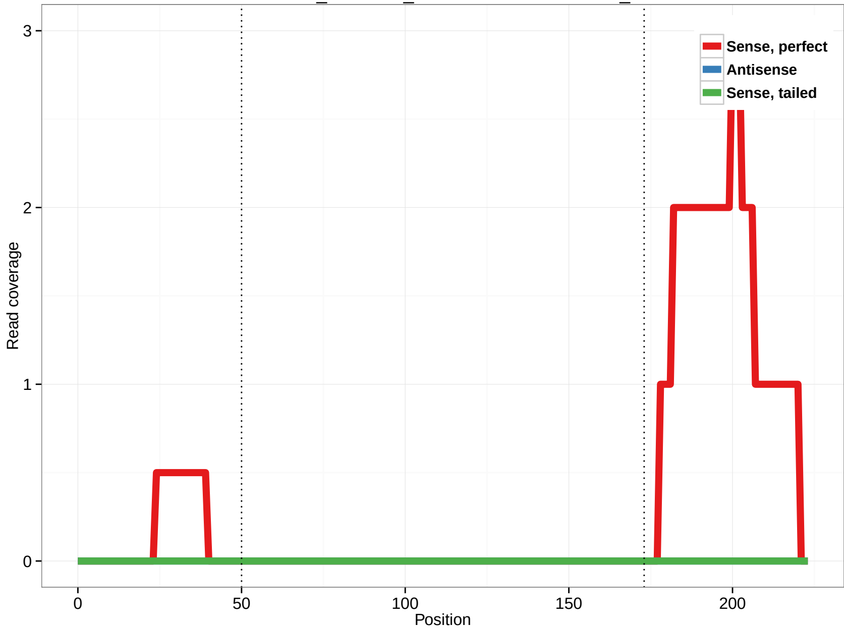
ornAna1_ensGene_ENSOANT00000030195_2
