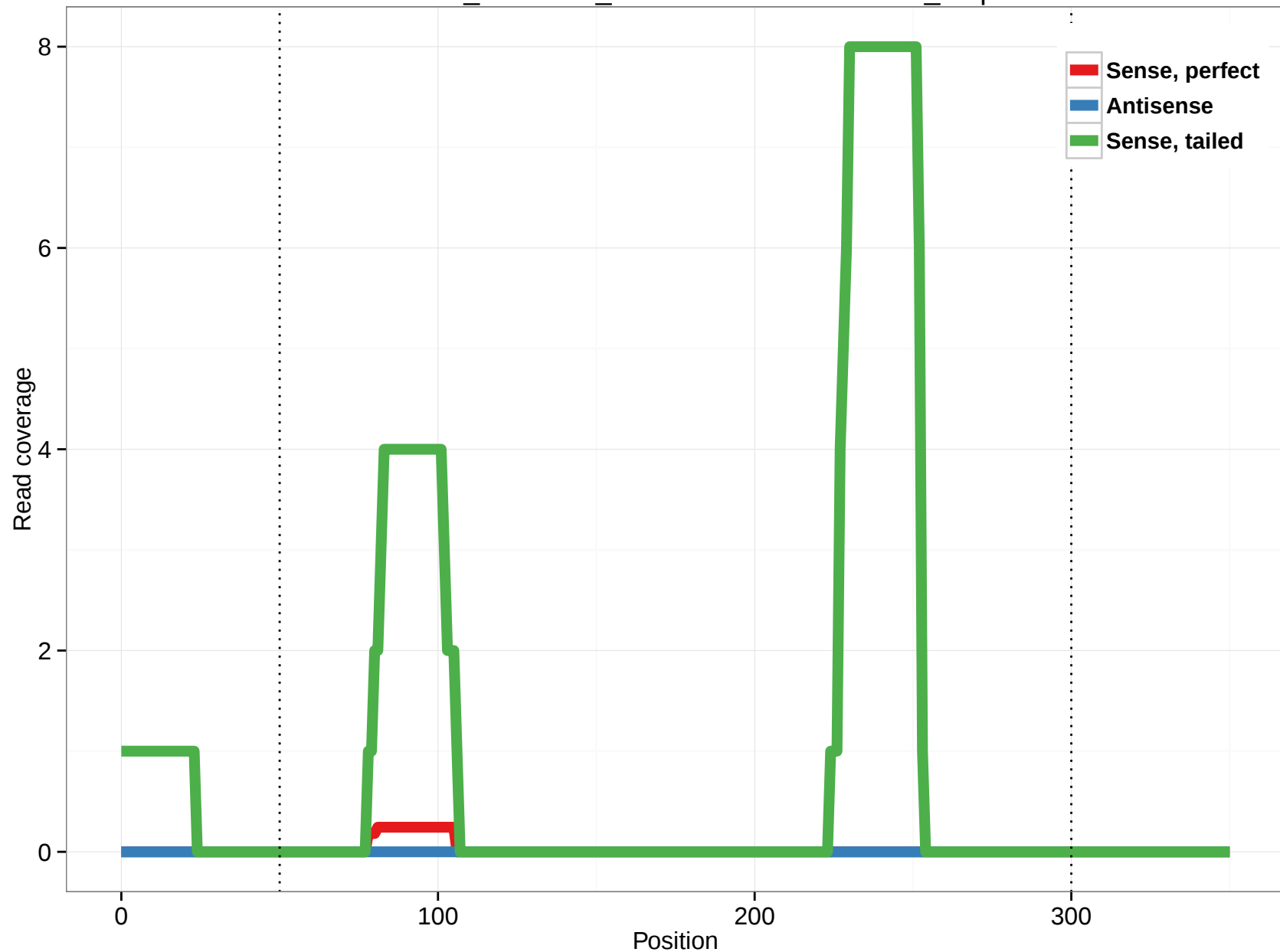
ornAna1_ensGene_ENSOANT00000030091_0.3p
