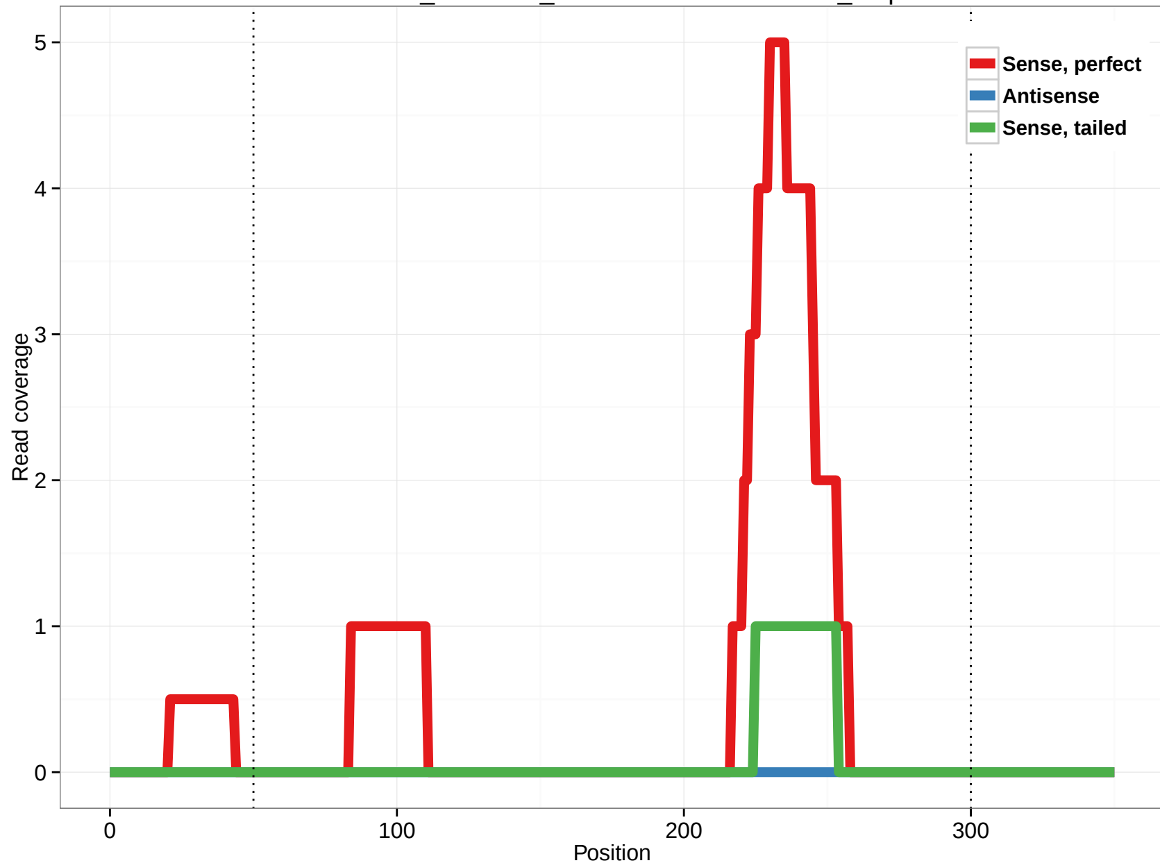
ornAna1_ensGene_ENSOANT00000030044_4.3p
