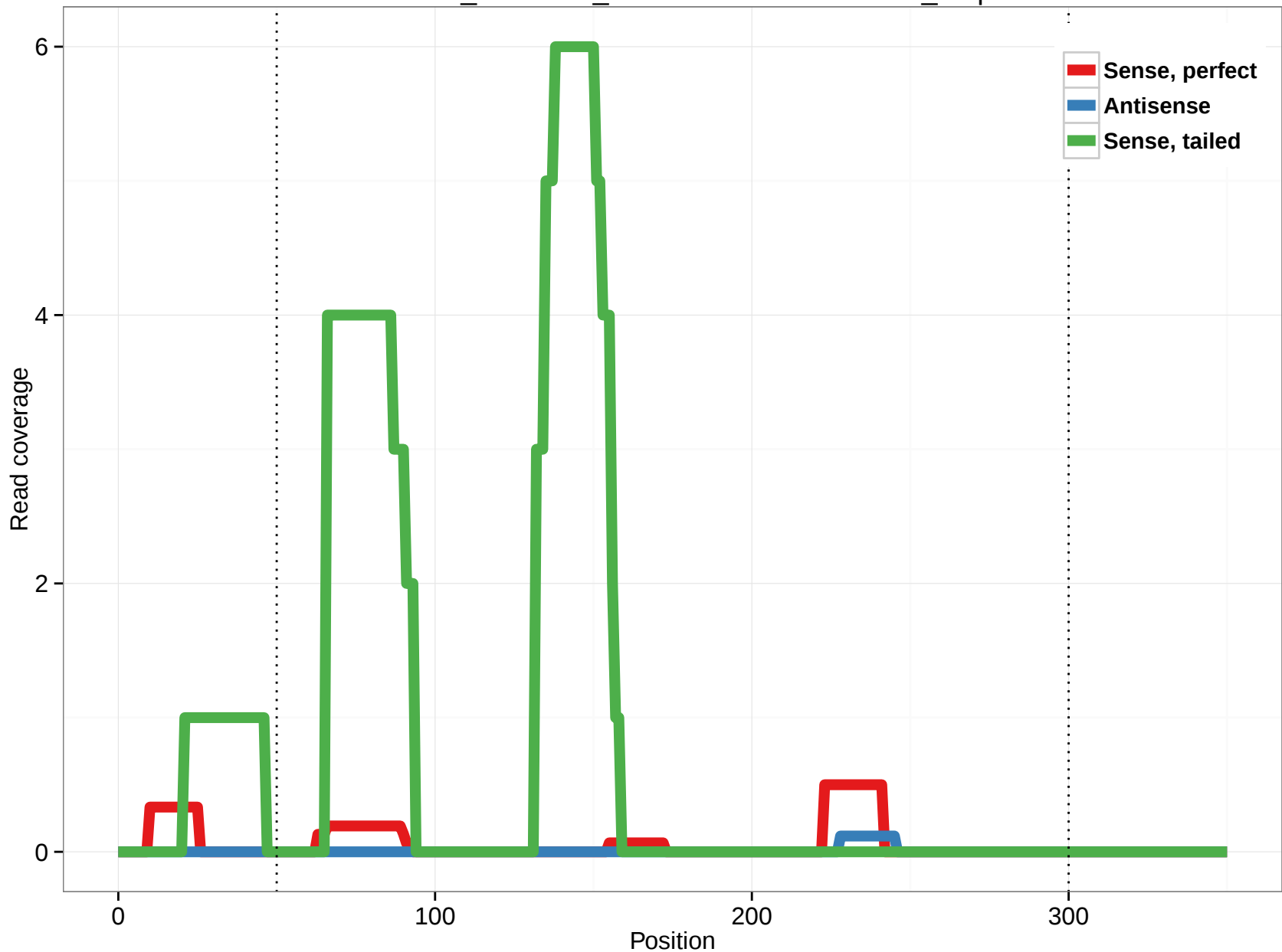
ornAna1_ensGene_ENSOANT00000029961_2.3p
