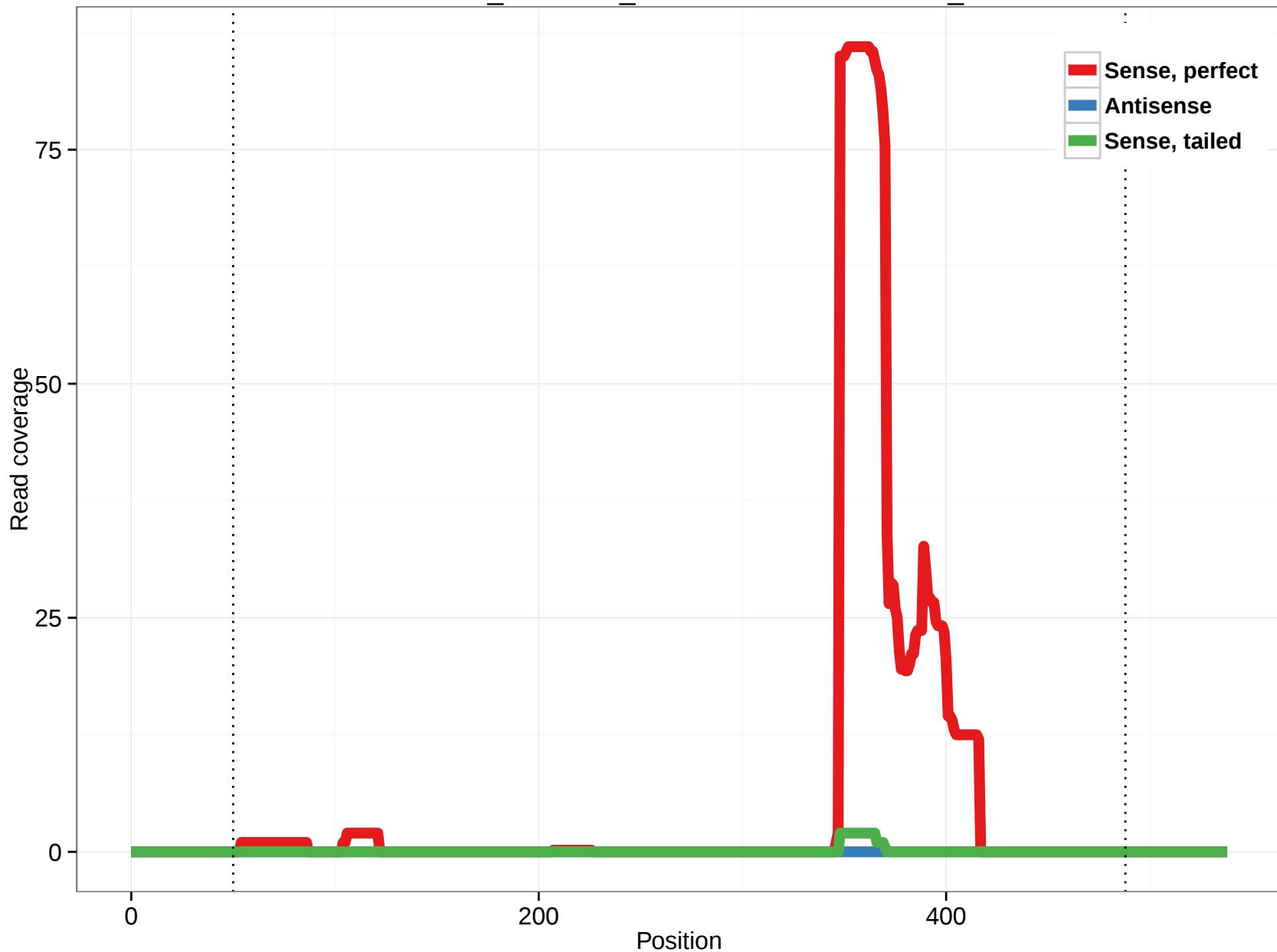
ornAna1_ensGene_ENSOANT00000029860_3
