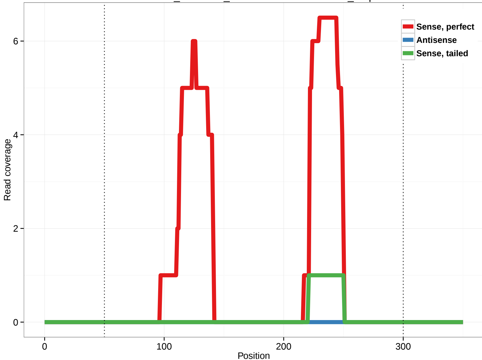
ornAna1_ensGene_ENSOANT00000029806_8.5p
