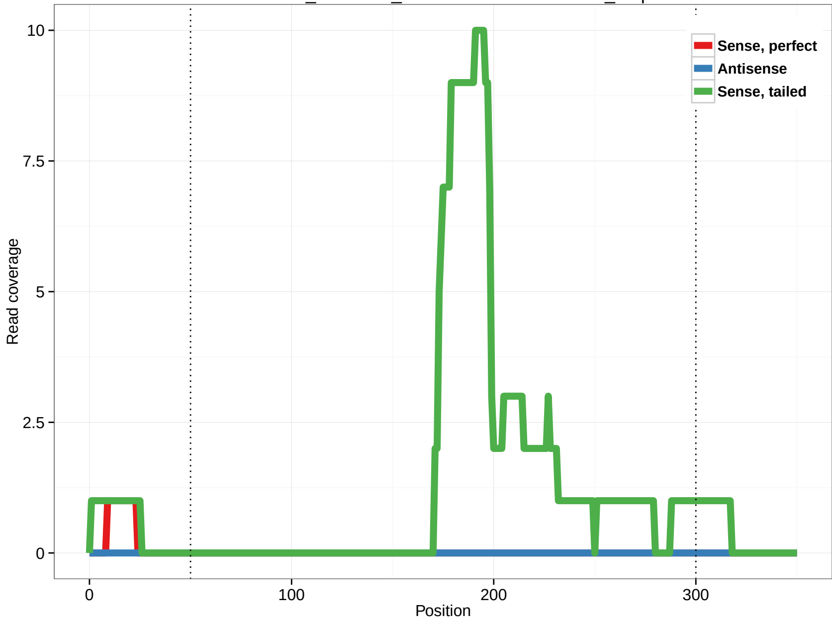
ornAna1_ensGene_ENSOANT00000029712_6.5p
