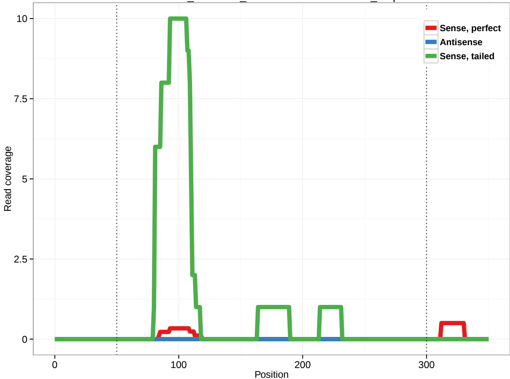
ornAna1_ensGene_ENSOANT00000029707_5.3p
