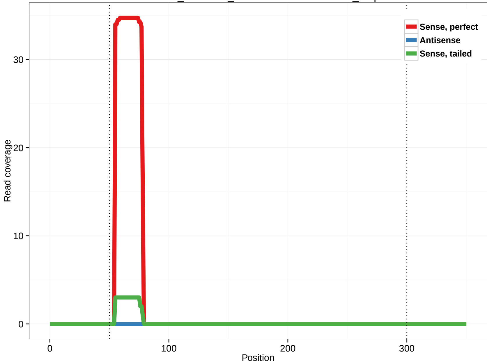
ornAna1_ensGene_ENSOANT00000029614_2.3p
