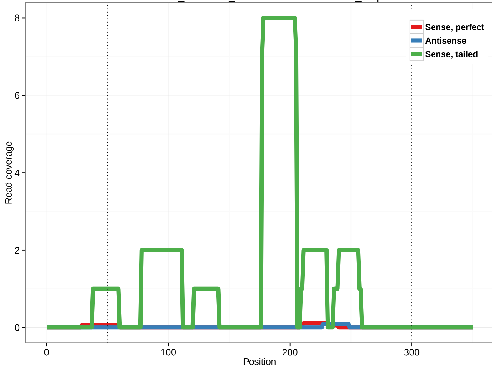
ornAna1_ensGene_ENSOANT00000029535_8.3p
