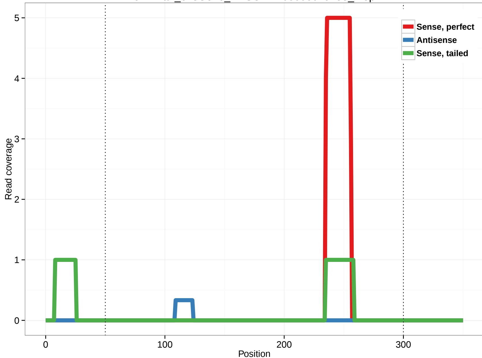
ornAna1_ensGene_ENSOANT00000029298_2.3p
