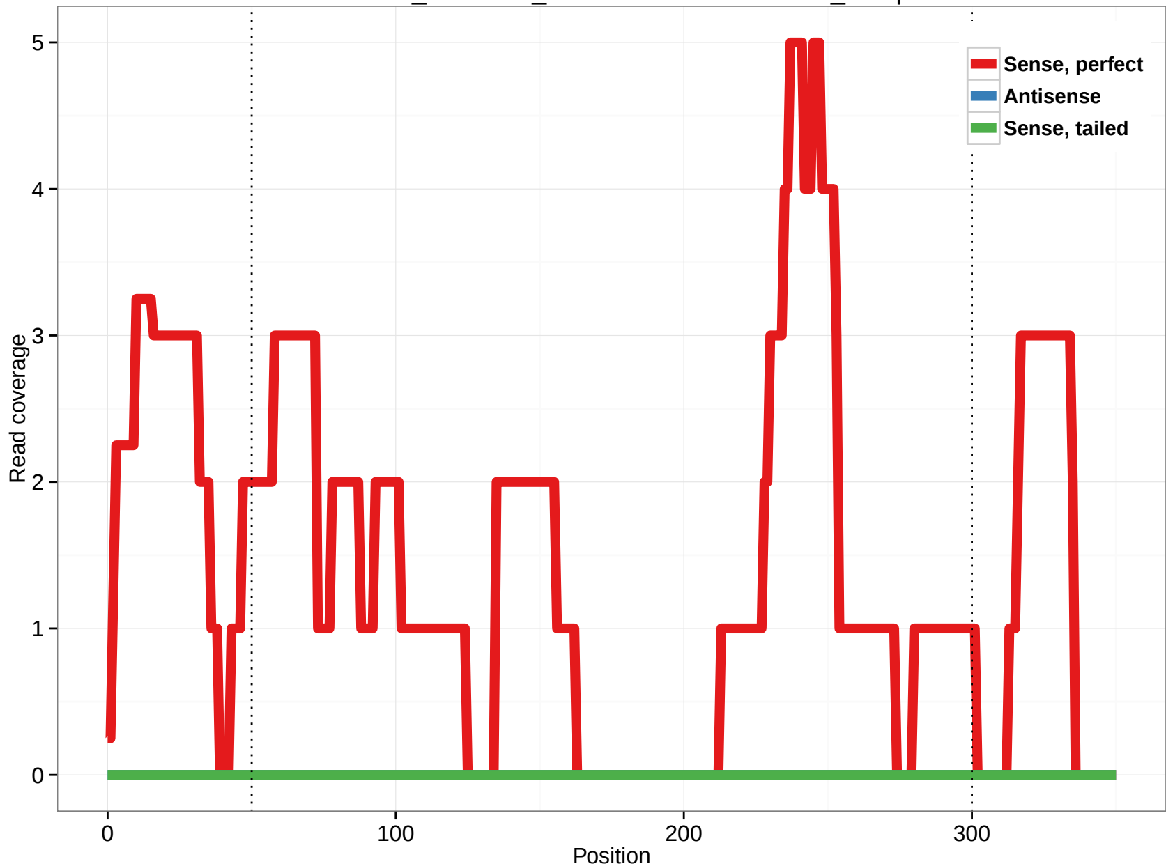
ornAna1_ensGene_ENSOANT00000029160_15.3p
