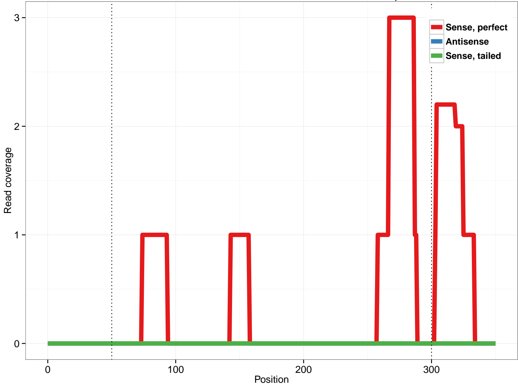
ornAna1_ensGene_ENSOANT00000029154_0.3p
